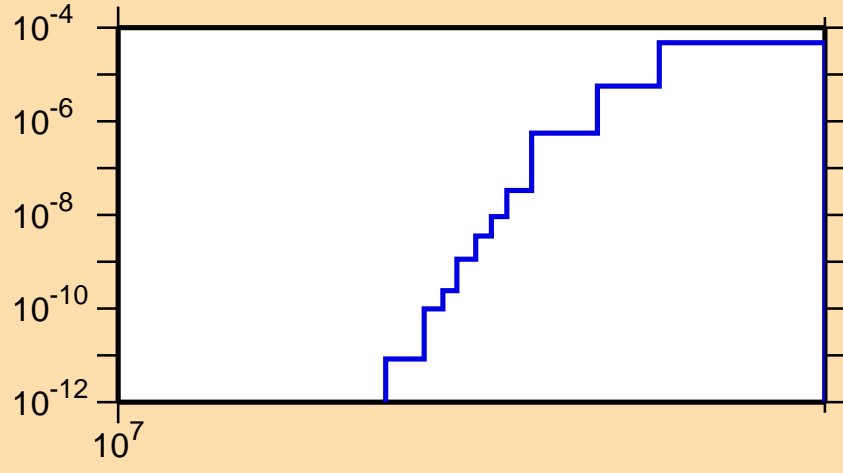
\sigma vs. E for ^{63}\text{Fe}(n,\alpha)
