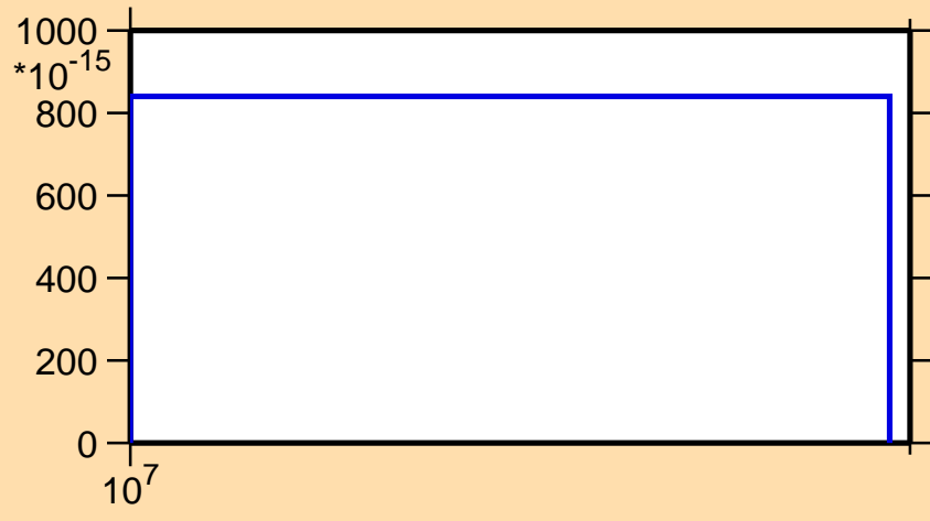
\sigma vs. E for ^{63}\text{Fe}(n,nt)
