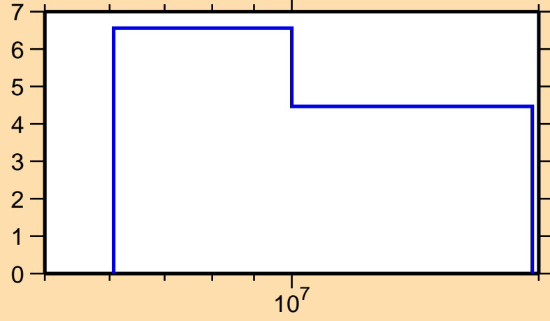
\Delta\sigma/\sigma vs. E for ^{63}\text{Fe}(n,\text{nonel.})
