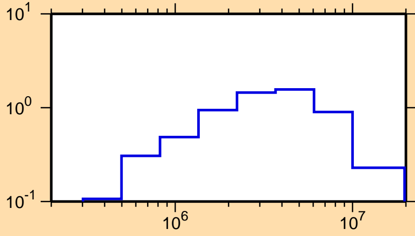
\sigma vs. E for ^{63}\text{Fe}(n,\text{inel.})
