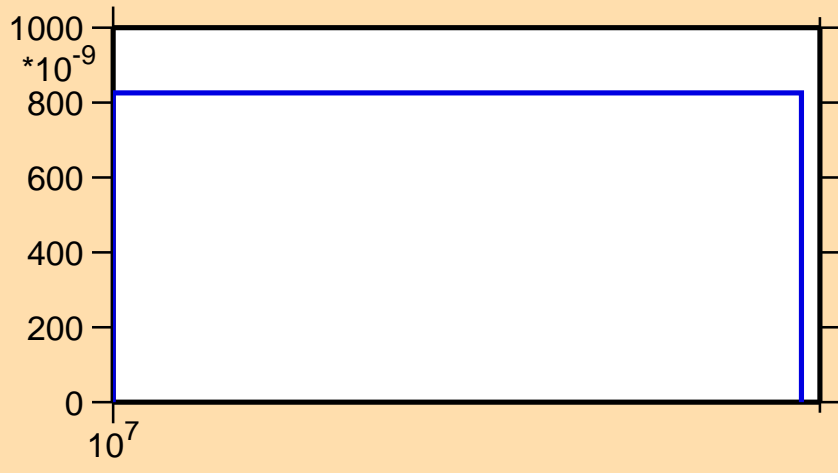
\sigma vs. E for ^{63}\text{Fe}(n,n\alpha)
