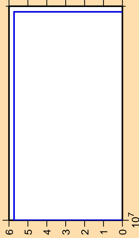
\Delta\sigma/\sigma vs. E for ^{63}\text{Fe}(n,3n)
