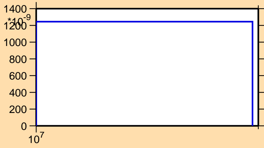
\sigma vs. E for ^{63}\text{Fe}(n,np)
