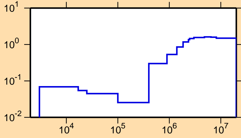
\sigma vs. E for ^{63}\text{Fe}(n,\text{nonel.})
