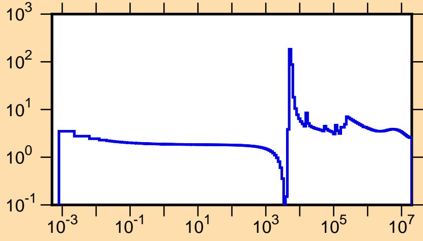
\sigma vs. E for ^{64}\text{Fe}(n,\text{tot.})
