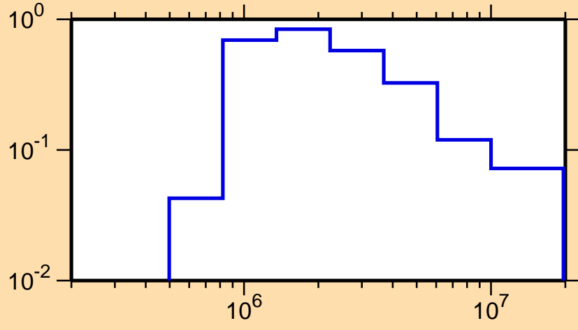
\sigma vs. E for ^{64}\text{Fe}(n,n_1)
