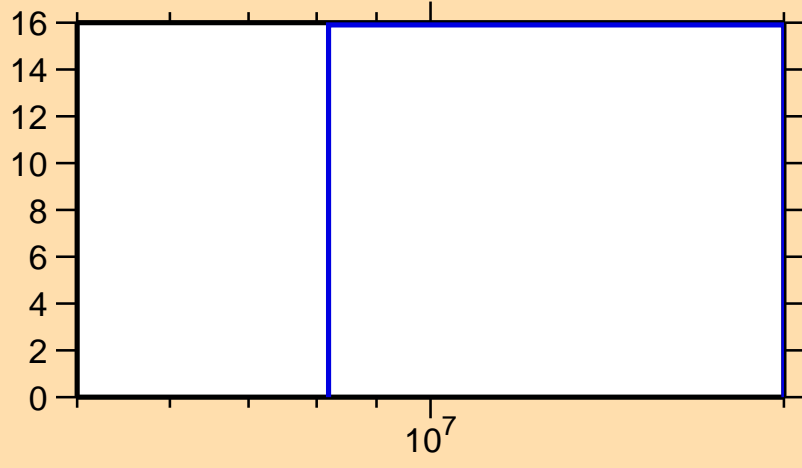
\Delta\sigma/\sigma vs. E for ^{64}\text{Fe}(n,el.)
