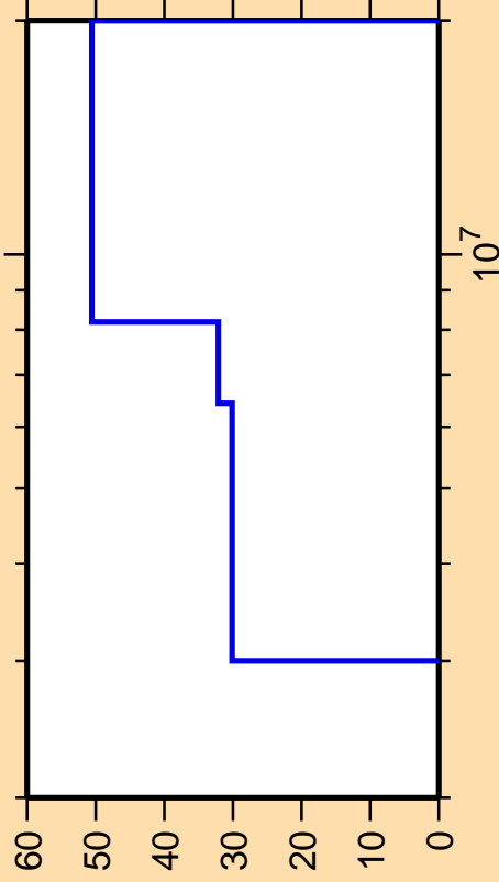
\Delta\sigma/\sigma vs. E for ^{64}\text{Fe}(n,\text{ncont.})
