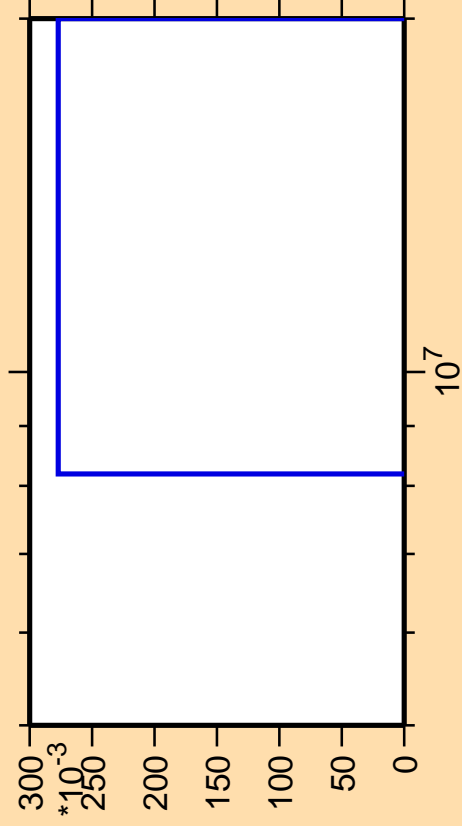
\Delta\sigma/\sigma vs. E for ^{64}\text{Fe}(n,nt)
