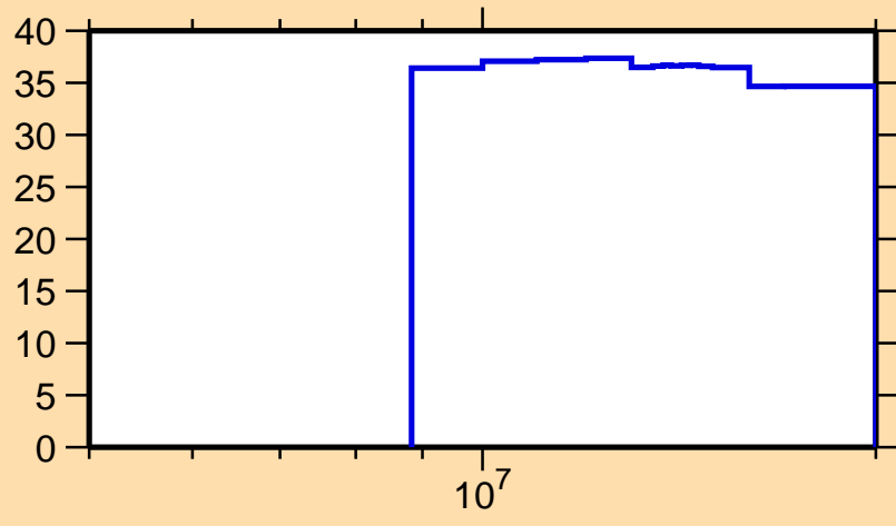
\Delta\sigma/\sigma vs. E for ^{65}\text{Fe}(n,ncont.)
