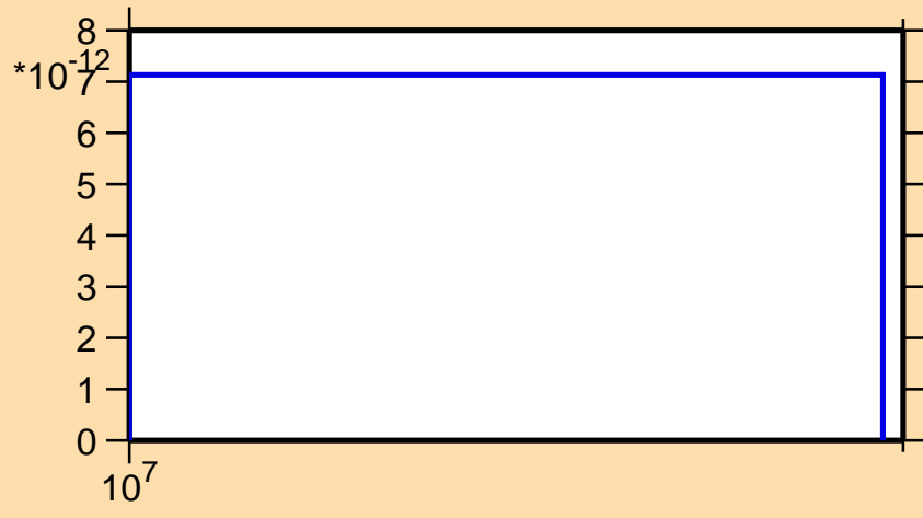
\sigma vs. E for ^{65}\text{Fe}(n,nt)
