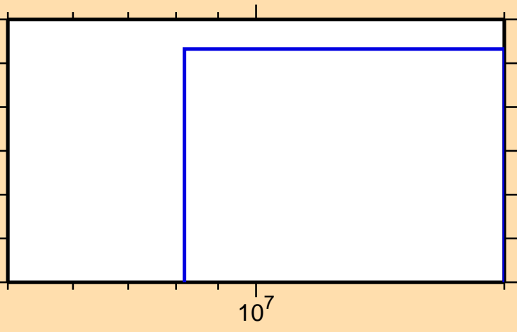
\sigma vs. E for ^{65}\text{Fe}(n,nt)
