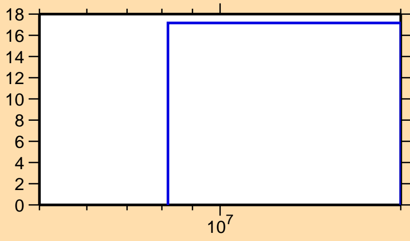
\Delta\sigma/\sigma vs. E for ^{65}\text{Fe}(n,el.)
