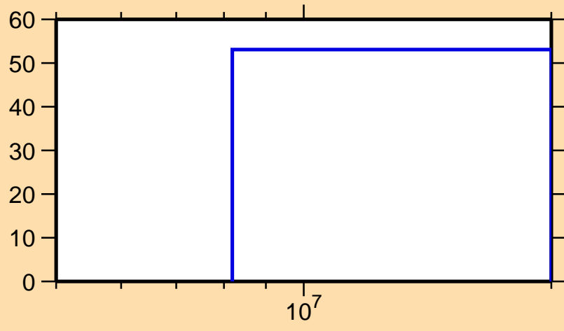
\Delta\sigma/\sigma vs. E for ^{65}\text{Fe}(n,p)
