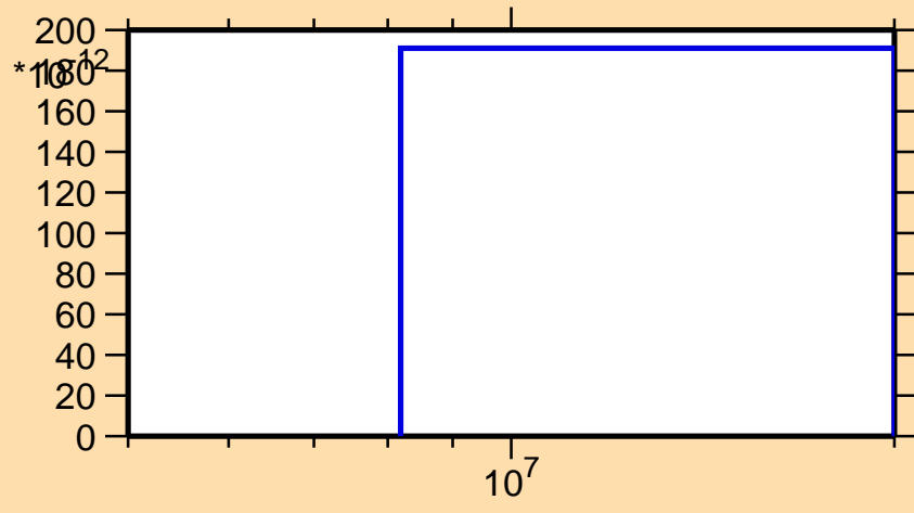
\sigma vs. E for ^{65}\text{Fe}(n,\text{nd})
