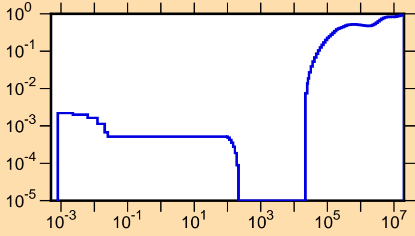
\mu vs. E for 289
