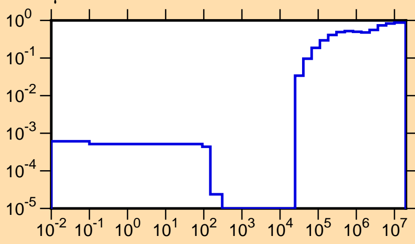
\mu vs. E for 289
