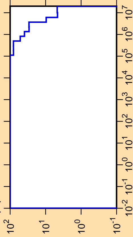
\Delta\mu/\mu vs. E for 289
