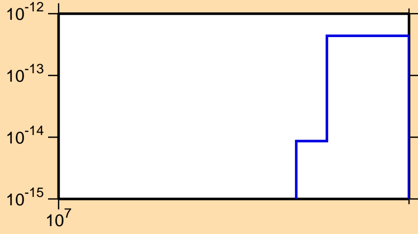
\sigma vs. E for ^{246}\text{Fm}(n,\text{pt})
