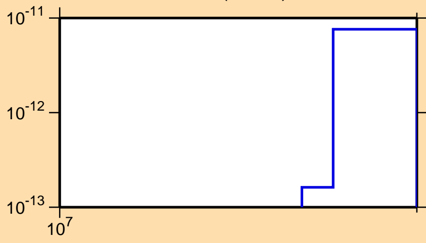
\sigma vs. E for ^{246}\text{Fm} (mt 34)
