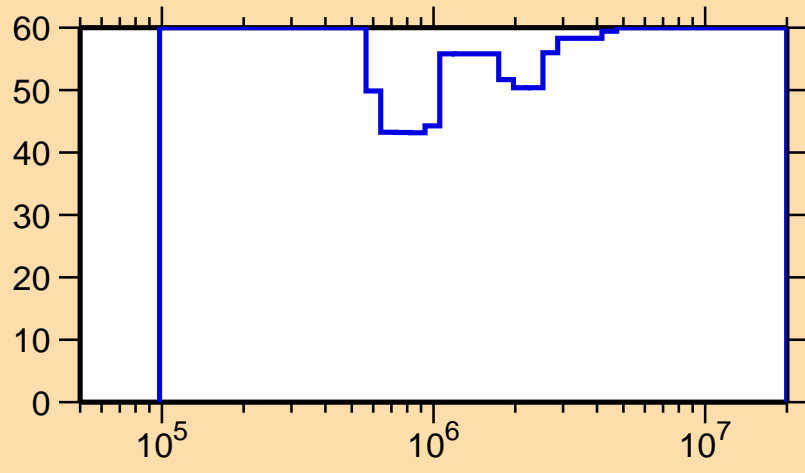
\Delta\sigma/\sigma vs. E for ^{246}\text{Fm}(n,\text{inel.})
