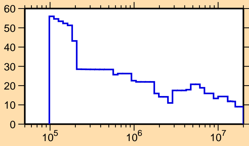
\Delta\sigma/\sigma vs. E for ^{246}\text{Fm}(n,tot.)
