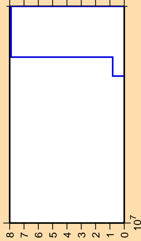
\Delta\sigma/\sigma vs. E for ^{246}\text{Fm}(n,\text{pd})
