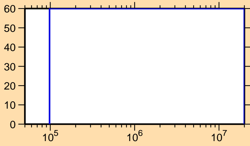
\Delta\sigma/\sigma vs. E for ^{246}\text{Fm}(n,ncont.)
