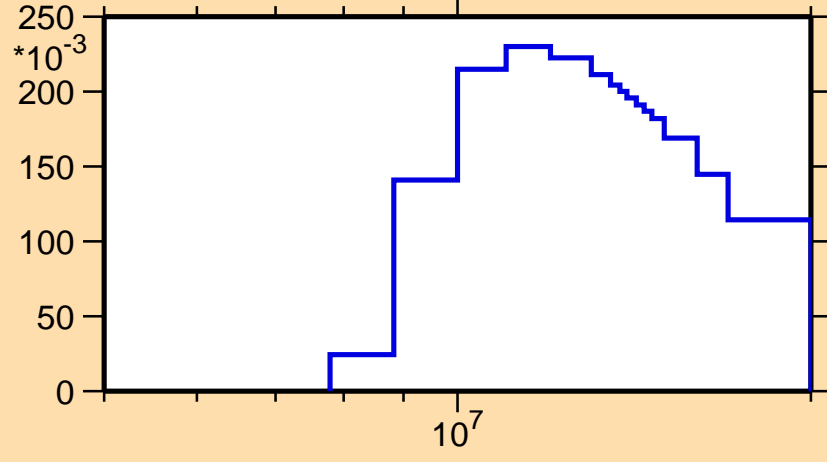
\sigma vs. E for ^{246}\text{Fm}(n,2n)
