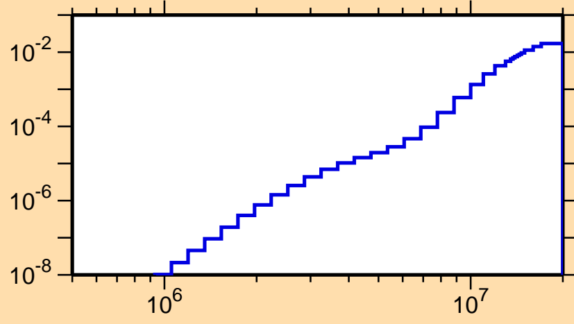
\sigma vs. E for ^{246}\text{Fm}(n,p)
