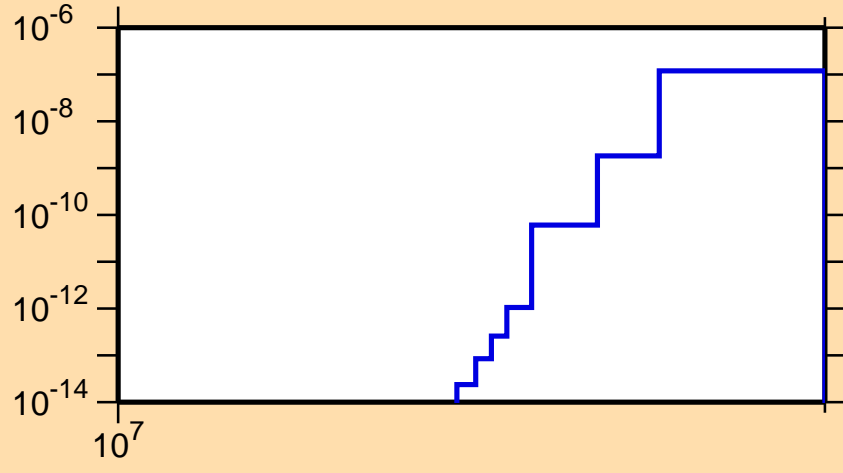
\sigma vs. E for ^{246}\text{Fm}(n,nt)
