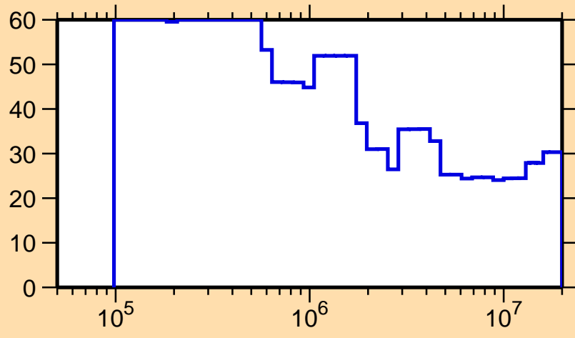
\Delta\sigma/\sigma vs. E for ^{246}\text{Fm}(n,n_1)
