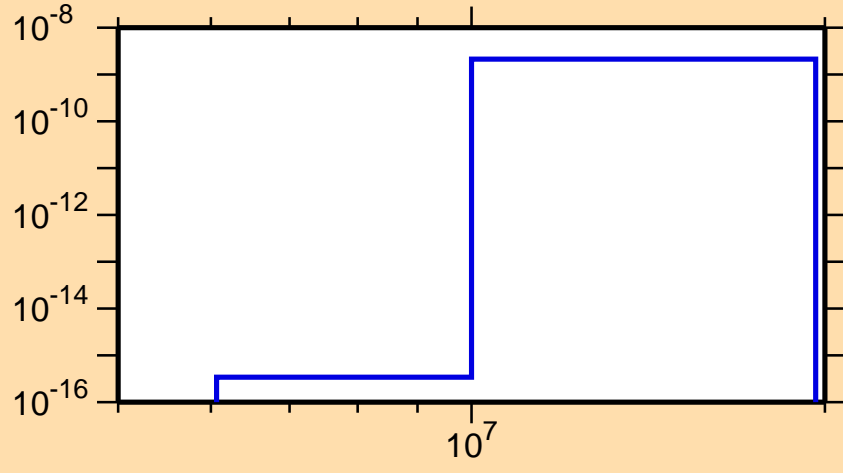
\sigma vs. E for ^{246}\text{Fm}(n,\text{He3})
