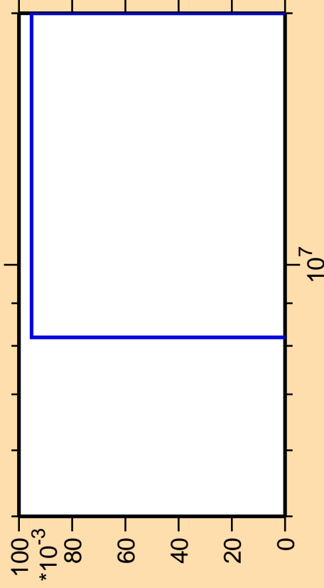
\Delta\sigma/\sigma vs. E for ^{246}\text{Fm}(n,\text{pd})
