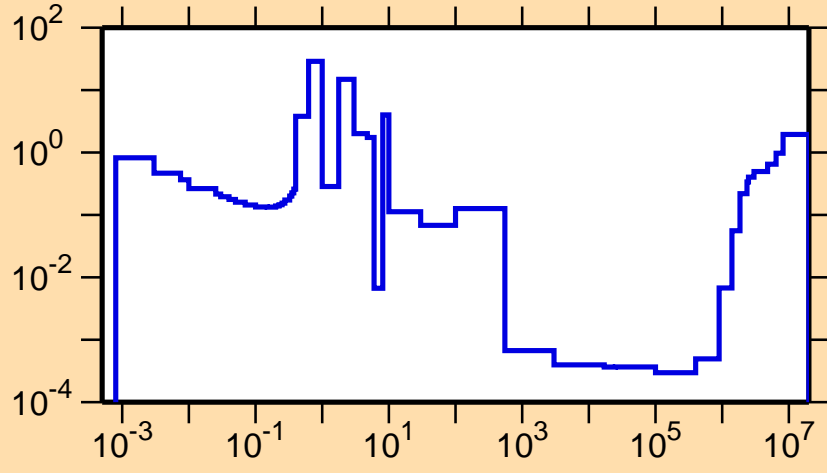
\sigma vs. E for ^{246}\text{Fm}(n,f)
