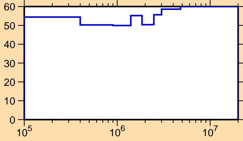
\Delta\sigma/\sigma vs. E for ^{246}\text{Fm}(n,inel.)
