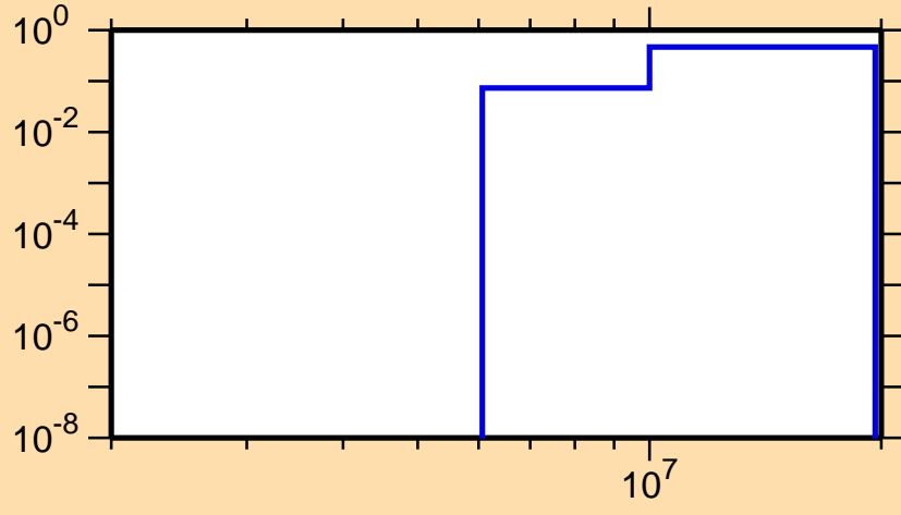
\sigma vs. E for ^{247}\text{Fm}(n,2n\alpha)
