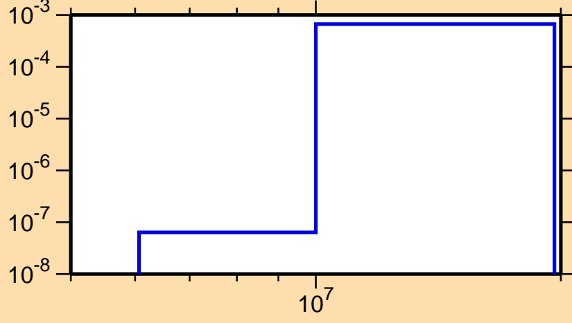
\sigma vs. E for ^{247}\text{Fm}(n,d)
