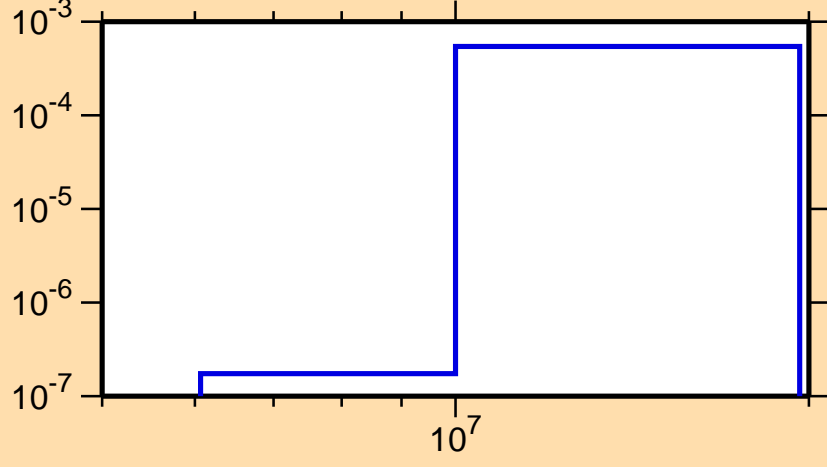
\sigma vs. E for ^{247}\text{Fm}(n,np)
