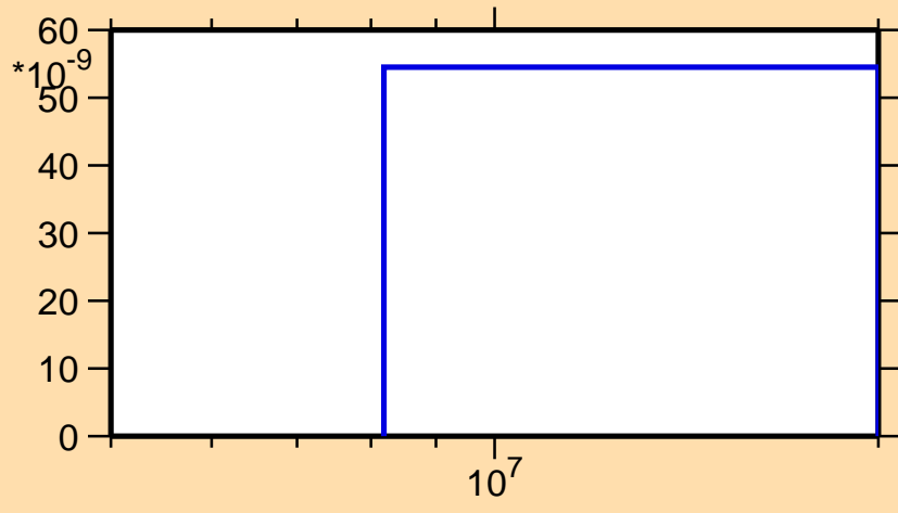
\sigma vs. E for ^{247}\text{Fm}(n,nd)
