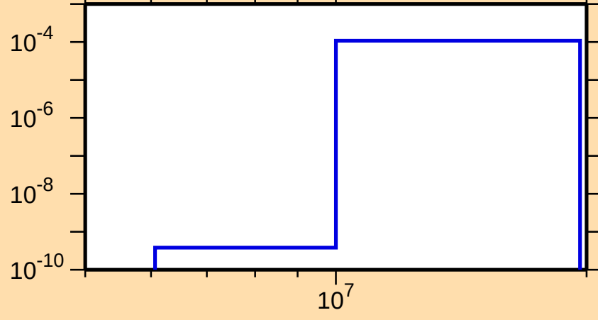
\sigma vs. E for ^{247}\text{Fm}(n,t)
