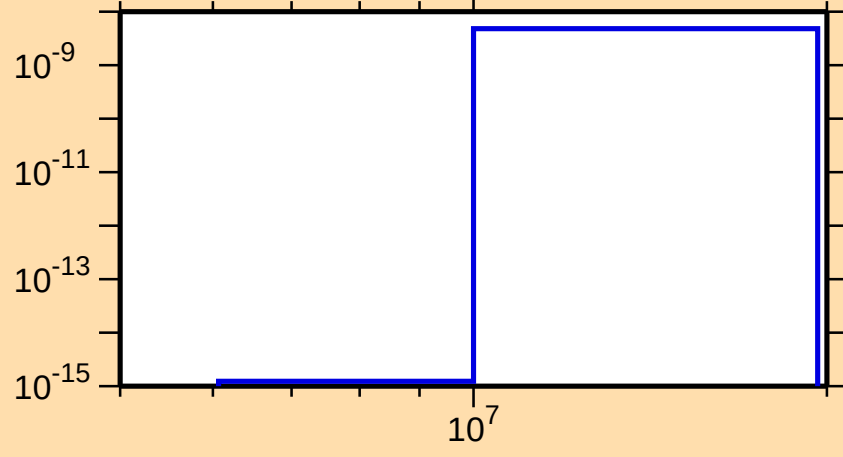
\sigma vs. E for ^{247}\text{Fm}(n,\text{He3})
