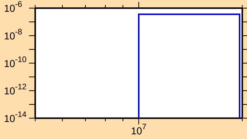
\sigma vs. E for ^{247}\text{Fm}(n,2np)
