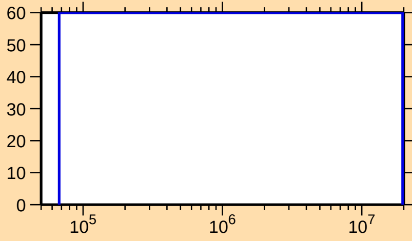
\Delta\sigma/\sigma vs. E for ^{247}\text{Fm}(n,n\text{cont.})
