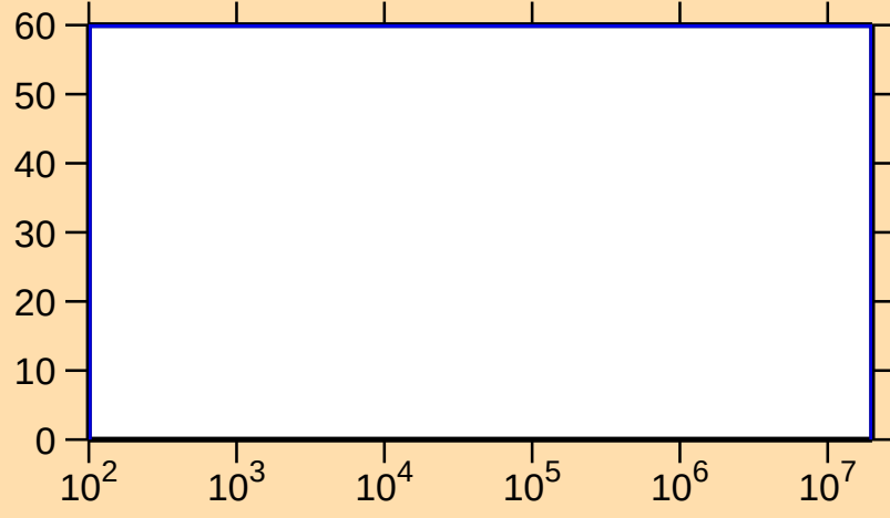
\Delta\sigma/\sigma vs. E for ^{247}\text{Fm}(n,\gamma)
