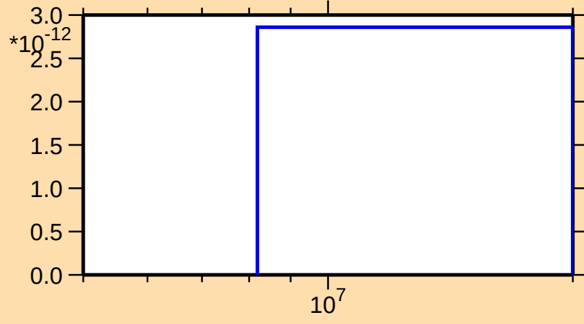
\sigma vs. E for ^{247}\text{Fm}(\text{mt } 34)
