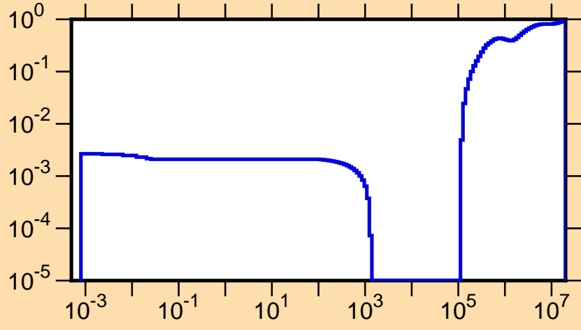
\mu vs. E for ^{248}\text{Fm}(\text{mt251})
