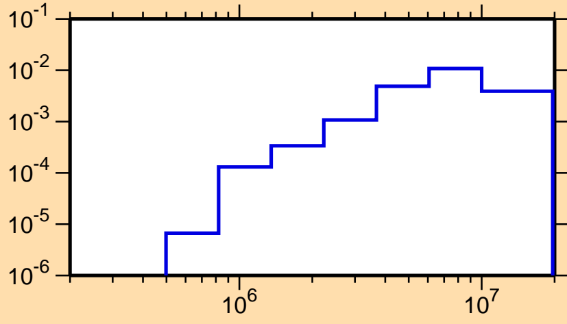
\sigma vs. E for ^{248}\text{Fm}(n,n\alpha)
