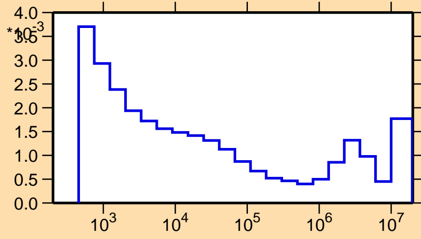
\sigma vs. E for ^{248}\text{Fm}(n,\alpha)
