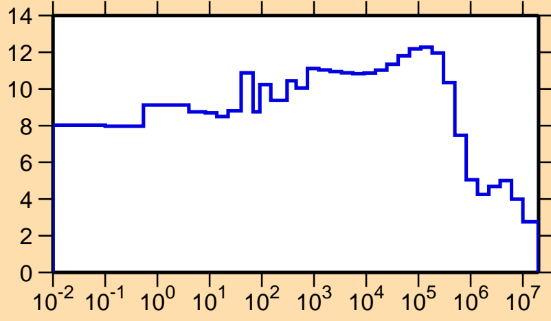
\sigma vs. E for ^{248}\text{Fm}(n,\text{el.})
