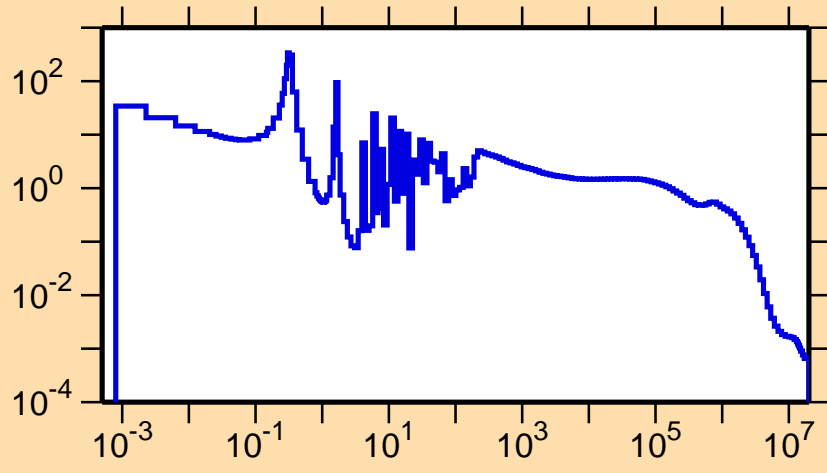
\sigma vs. E for ^{249}\text{Fm}(n,\gamma)
