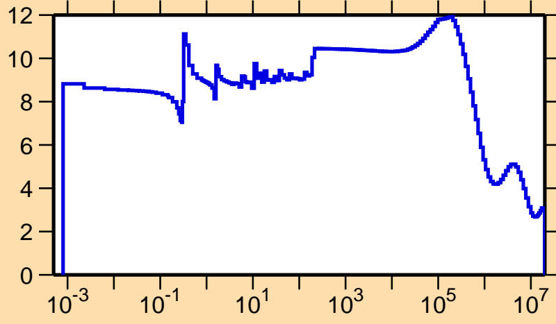
\sigma vs. E for ^{249}\text{Fm}(n,\text{el.})
