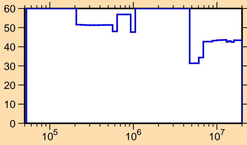
\Delta\sigma/\sigma vs. E for ^{249}\text{Fm}(n,n_1)
