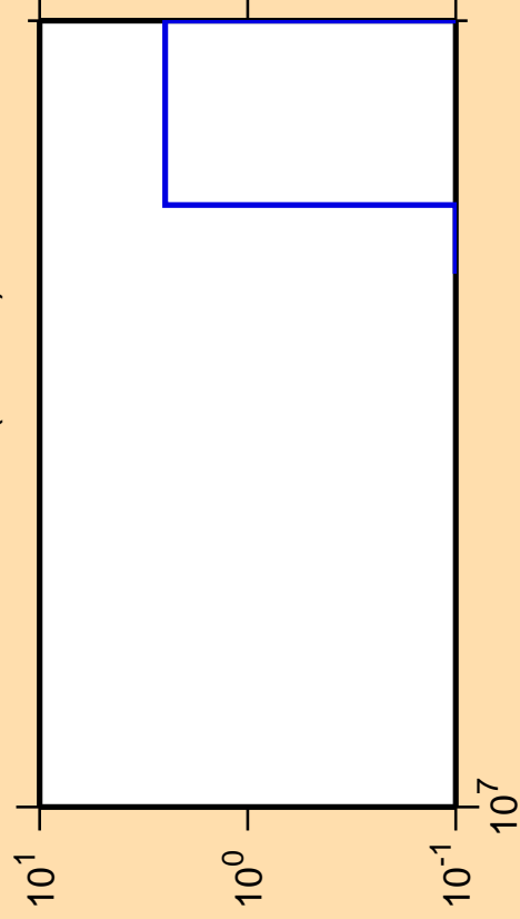
\Delta\sigma/\sigma vs. E for ^{249}\text{Fm} (mt 34)
