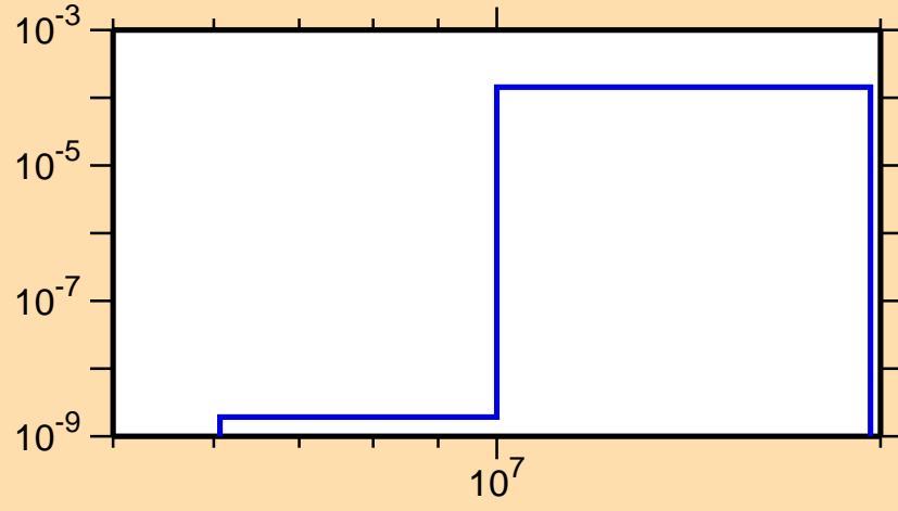
\sigma vs. E for ^{249}\text{Fm}(\text{mt117})
