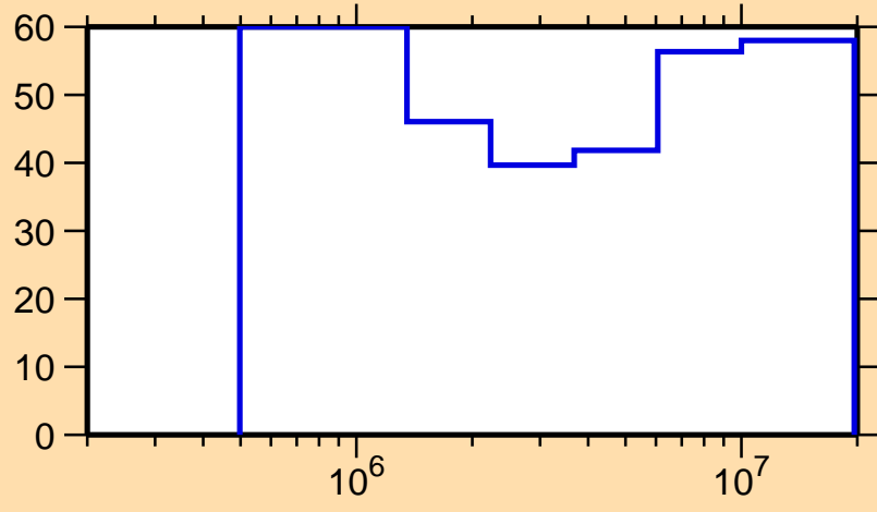
\Delta\sigma/\sigma vs. E for ^{249}\text{Fm}(n,ncont.)
