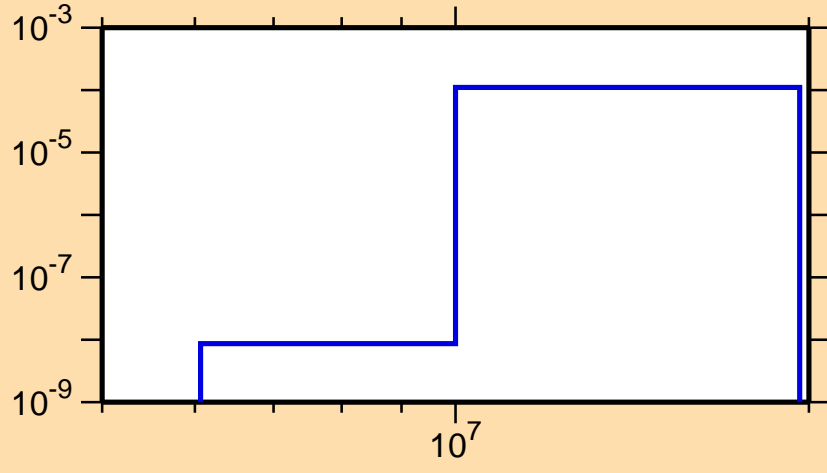
\sigma vs. E for ^{249}\text{Fm} (mt 45)
