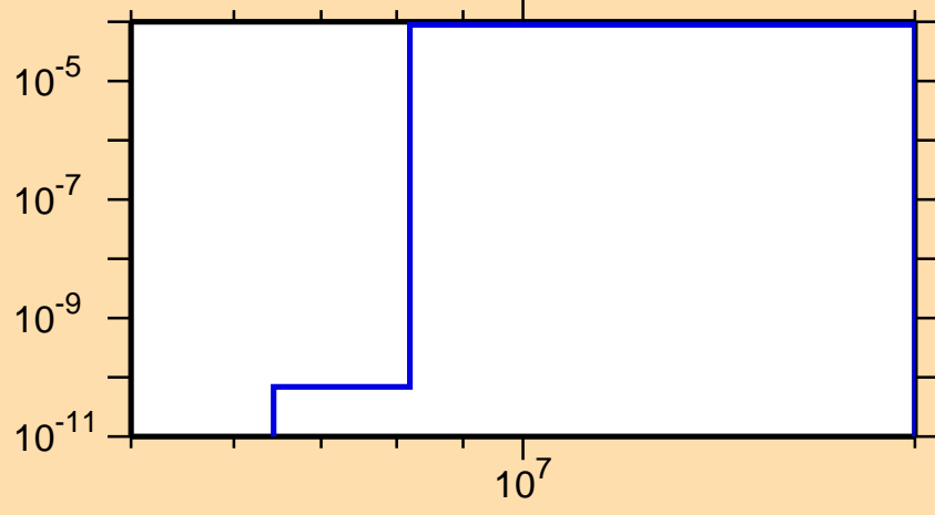
\sigma vs. E for ^{249}\text{Fm} (mt 45)
