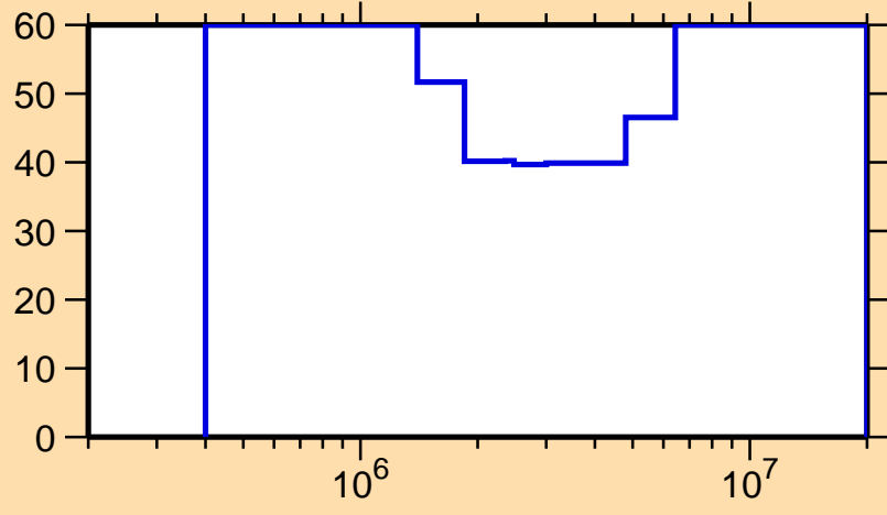
\Delta\sigma/\sigma vs. E for ^{249}\text{Fm}(n,n\text{cont.})
