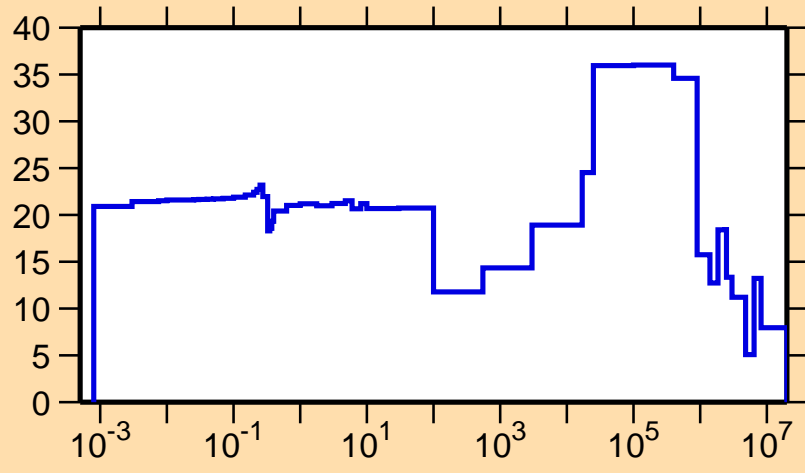
\Delta\sigma/\sigma vs. E for ^{249}\text{Fm}(n,el.)
