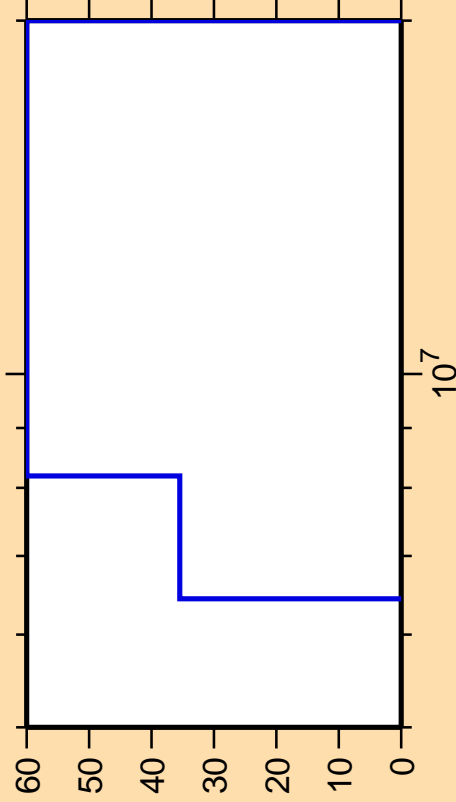
\Delta\sigma/\sigma vs. E for ^{249}\text{Fm} (mt 45)
