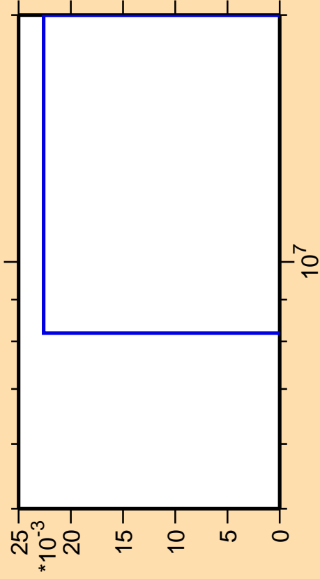
\Delta\sigma/\sigma vs. E for ^{249}\text{Fm} (mt 34)
