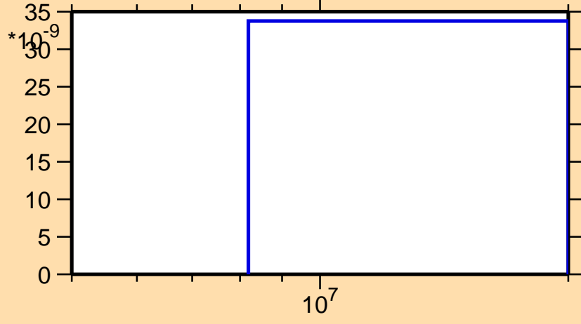
\sigma vs. E for ^{249}\text{Fm}(n,nd)
