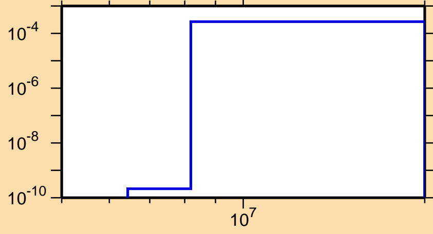
\sigma vs. E for ^{249}\text{Fm}(n,np)
