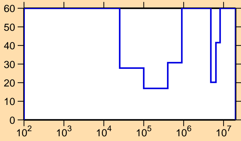
\Delta\sigma/\sigma vs. E for ^{249}\text{Fm}(n,p)
