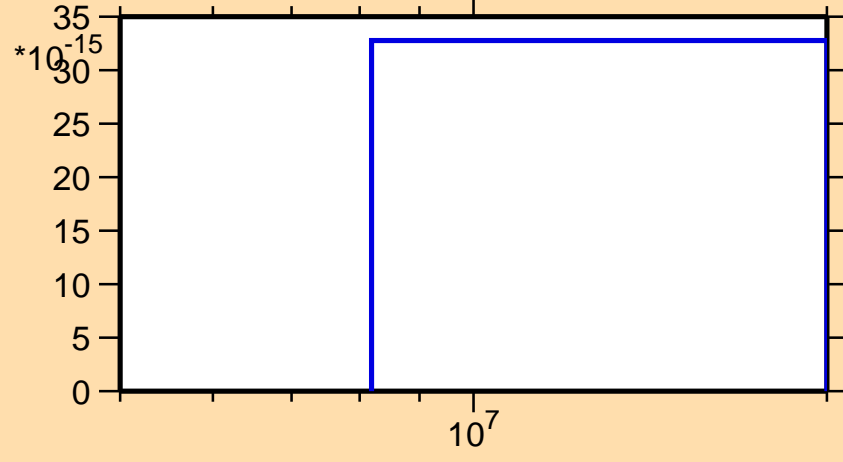
\sigma vs. E for ^{249}\text{Fm} (mt 34)
