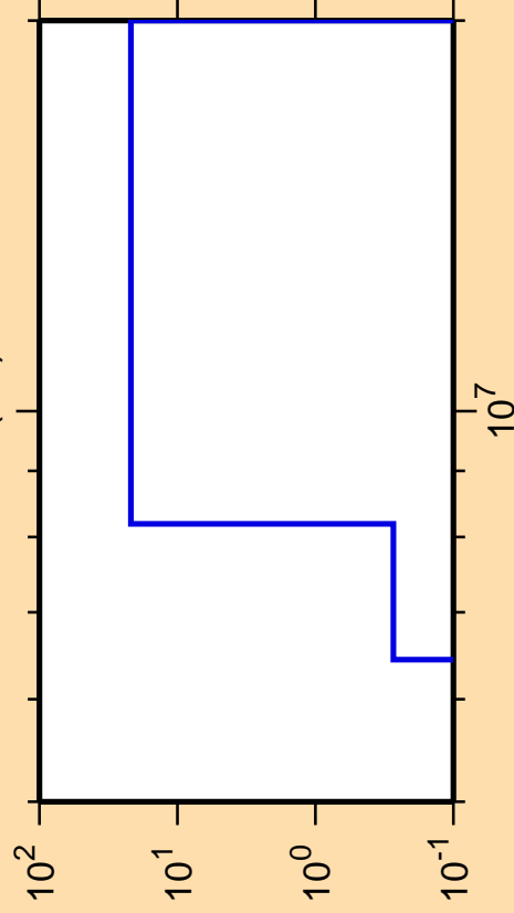
\Delta\sigma/\sigma vs. E for ^{249}\text{Fm}(n,t)
