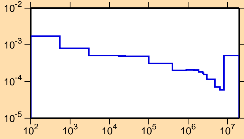
\sigma vs. E for ^{249}\text{Fm}(n,\alpha)
