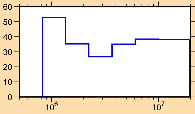
\Delta\sigma/\sigma vs. E for ^{250}\text{Fm}(n,ncont.)
