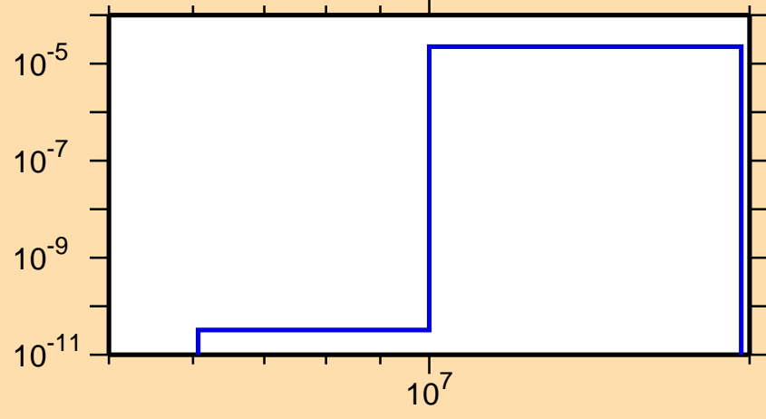
\sigma vs. E for ^{250}\text{Fm}(\text{mt117})
