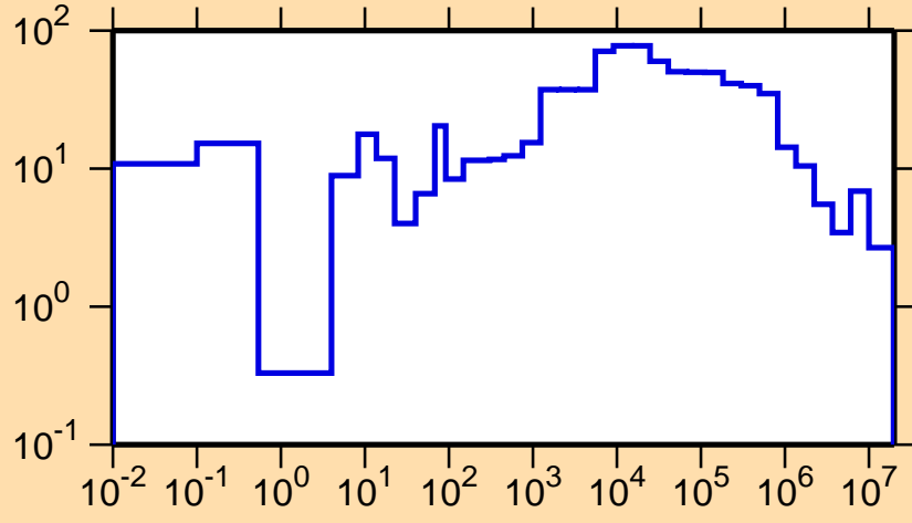
\Delta\sigma/\sigma vs. E for ^{250}\text{Fm}(n,tot.)
