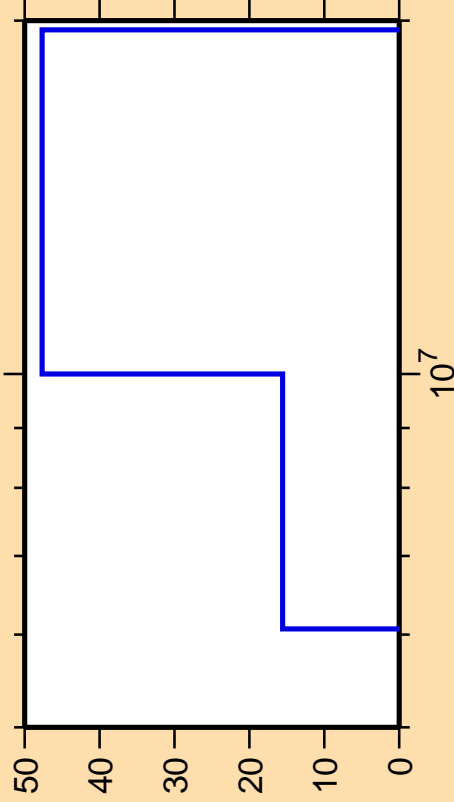
\Delta\sigma/\sigma vs. E for ^{250}\text{Fm}(\text{mt117})
