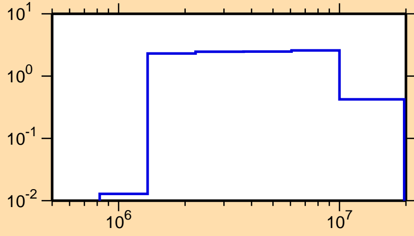
\sigma vs. E for ^{250}\text{Fm}(n,\text{inel.})
