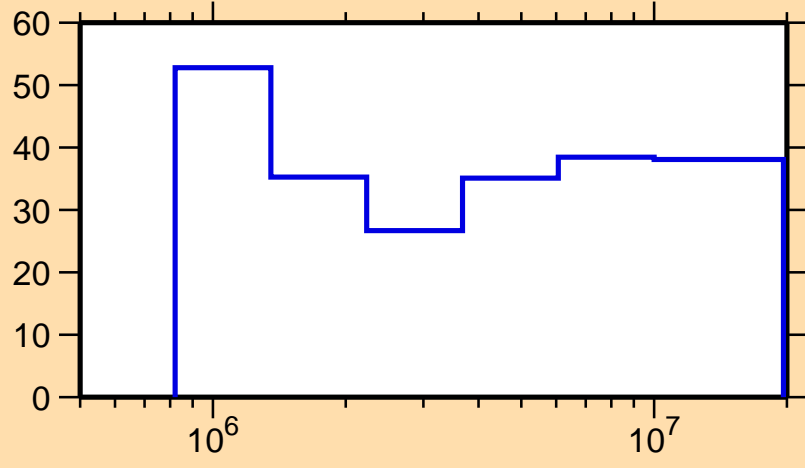
\Delta\sigma/\sigma vs. E for ^{250}\text{Fm}(n,ncont.)
