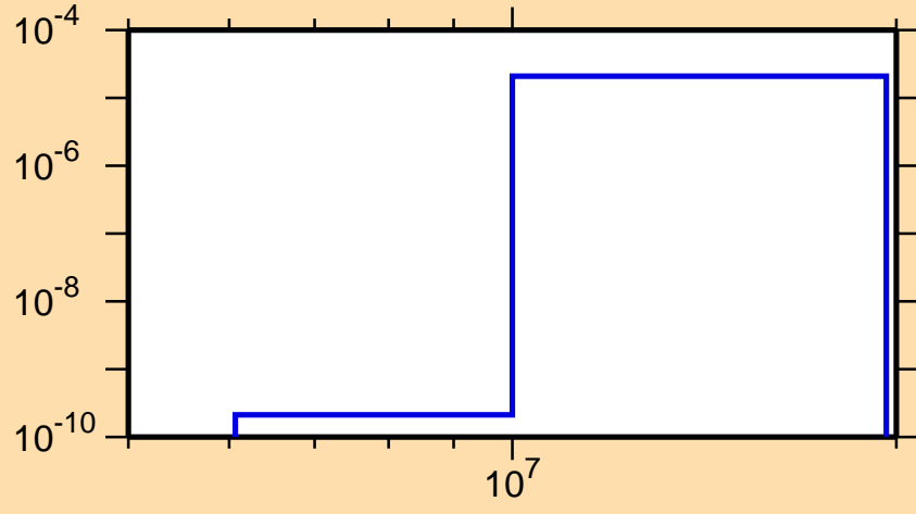
\sigma vs. E for ^{250}\text{Fm} (mt 45)
