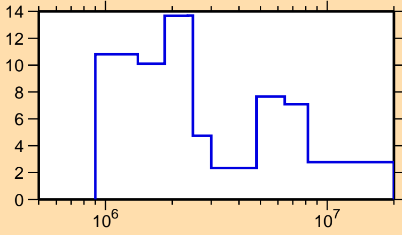
\Delta\sigma/\sigma vs. E for ^{250}\text{Fm}(n,tot.)
