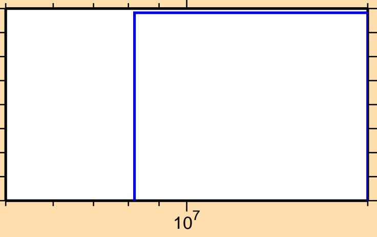
\sigma vs. E for ^{250}\text{Fm}(n,3n)
