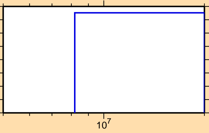
\sigma vs. E for ^{250}\text{Fm} (mt 34)
