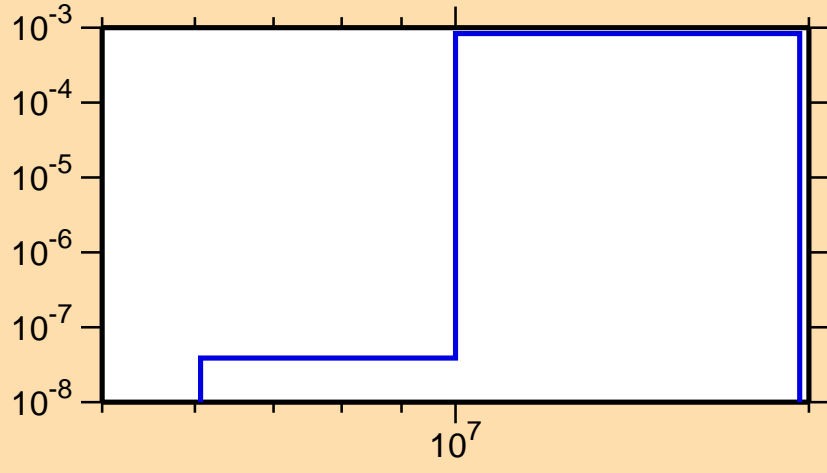
\sigma vs. E for ^{250}\text{Fm}(n,d)
