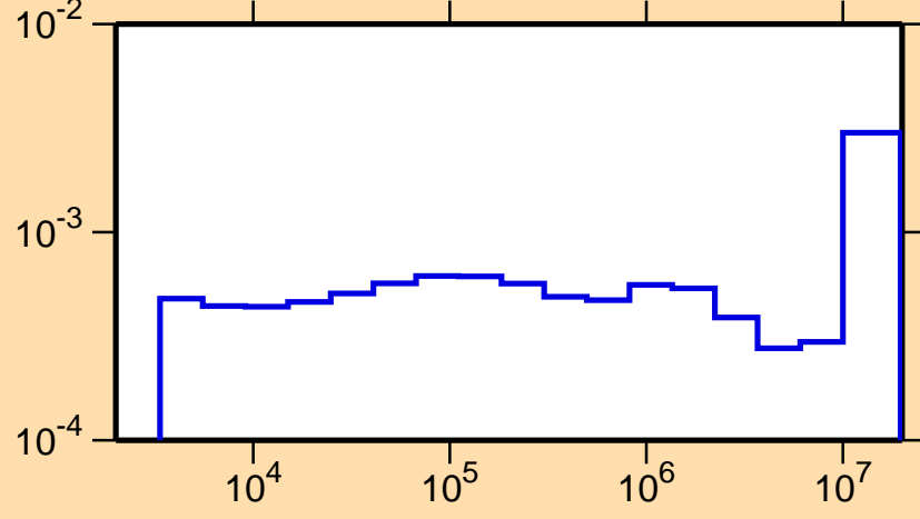
\sigma vs. E for ^{250}\text{Fm}(n,\alpha)
