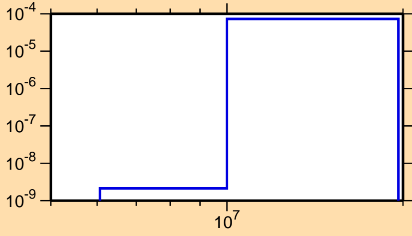
\sigma vs. E for ^{250}\text{Fm}(\text{mt117})
