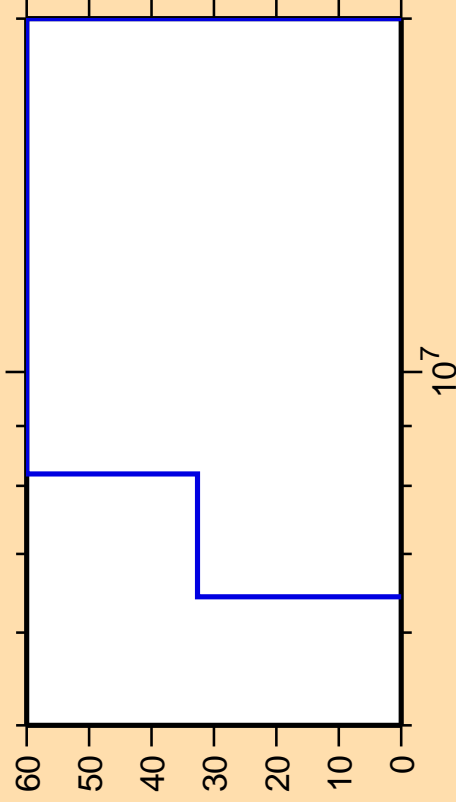
\Delta\sigma/\sigma vs. E for ^{250}\text{Fm}(\text{mt117})
