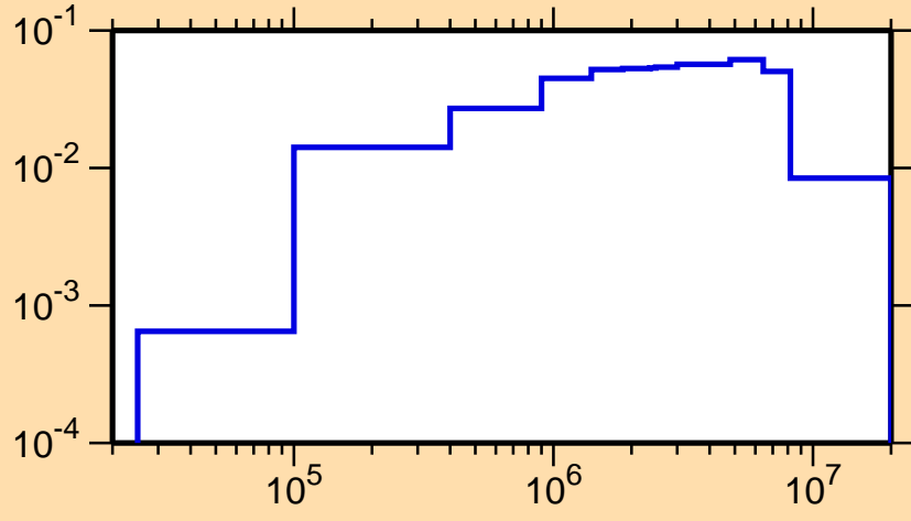
\sigma vs. E for ^{250}\text{Fm}(n,n\alpha)
