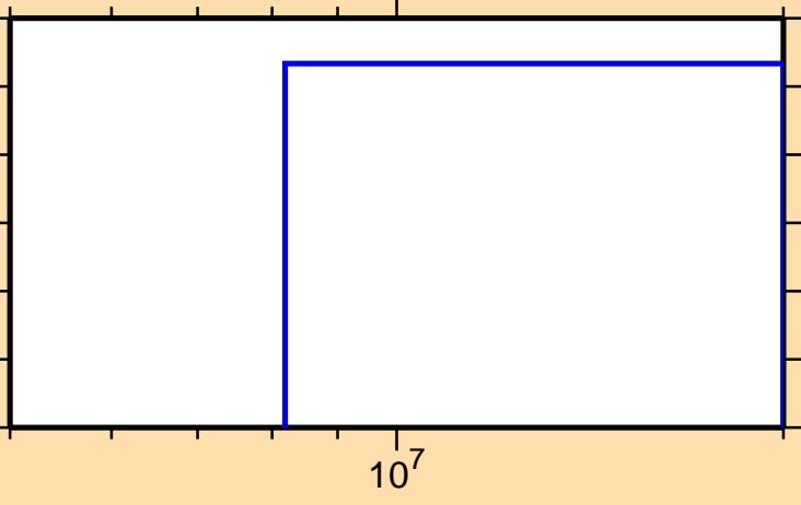
\sigma vs. E for ^{250}\text{Fm}(n,nd)
