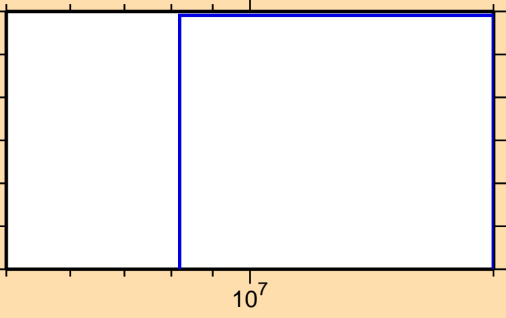
\sigma vs. E for ^{250}\text{Fm}(n,2np)
