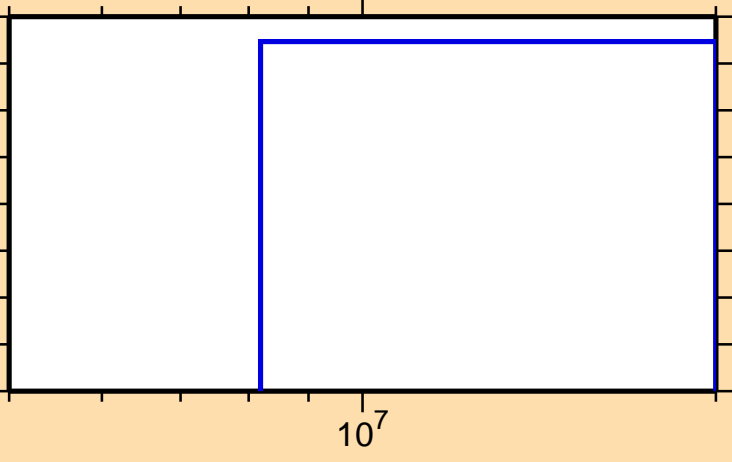
\sigma vs. E for ^{251}\text{Fm}(n,3n)
