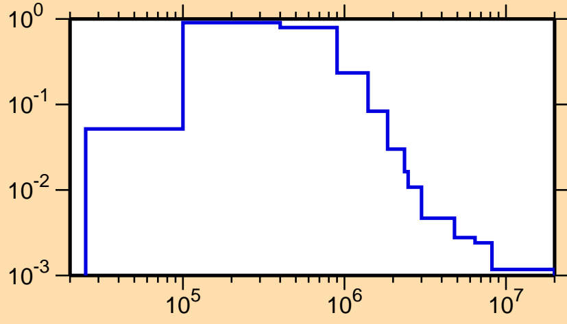
\sigma vs. E for ^{251}\text{Fm}(n,n_1)
