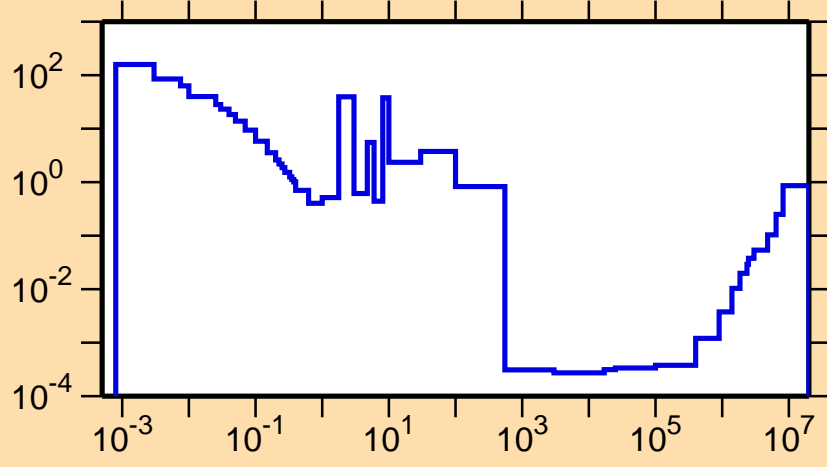
\sigma vs. E for ^{251}\text{Fm}(n,f)
