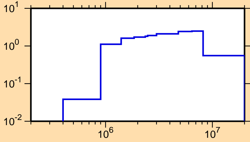
\sigma vs. E for ^{251}\text{Fm}(n,n\text{cont.})
