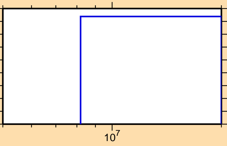
\sigma vs. E for ^{251}\text{Fm} (mt 34)
