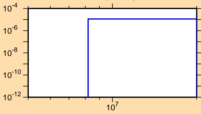
\sigma vs. E for ^{251}\text{Fm} (mt 45)
