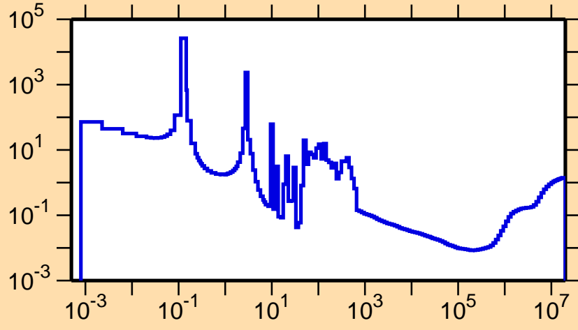
\sigma vs. E for ^{253}\text{Fm}(n,f)
