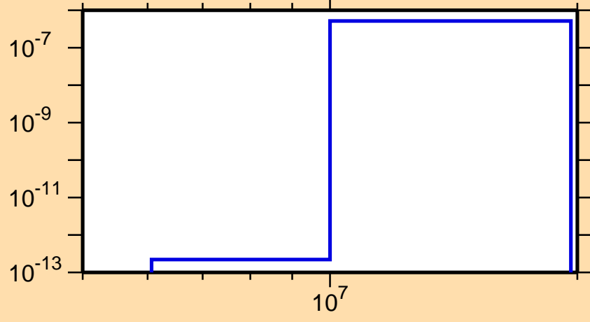
\sigma vs. E for ^{253}\text{Fm}(\text{mt117})
