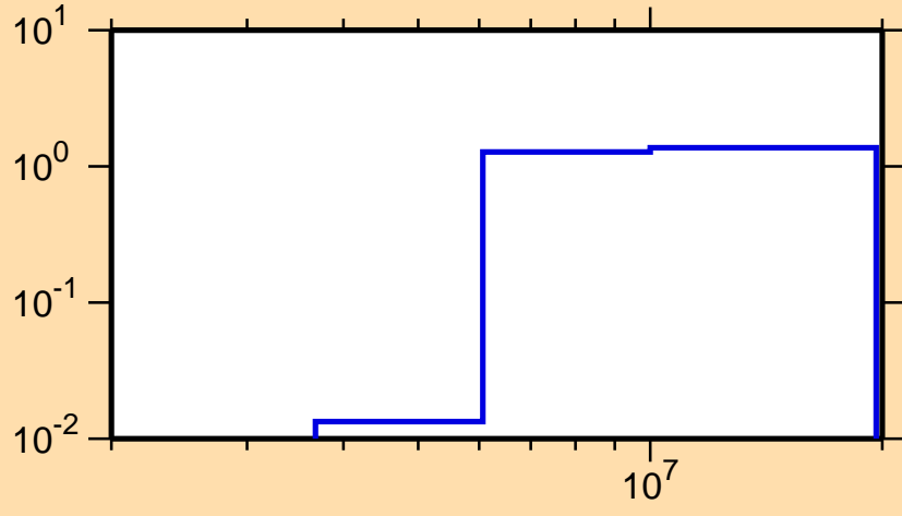
\sigma vs. E for ^{253}\text{Fm}(n,2n)
