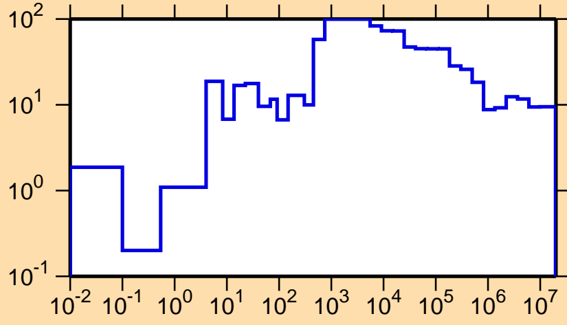
\Delta\sigma/\sigma vs. E for ^{253}\text{Fm}(n,tot.)
