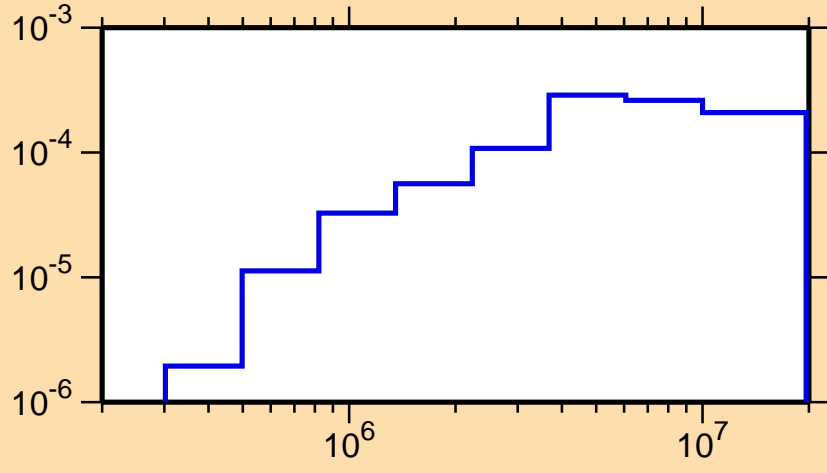
\sigma vs. E for ^{253}\text{Fm}(n,n\alpha)
