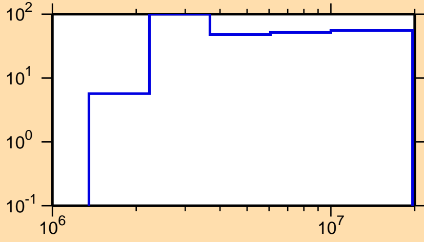
\Delta\sigma/\sigma vs. E for ^{253}\text{Fm}(n,p)
