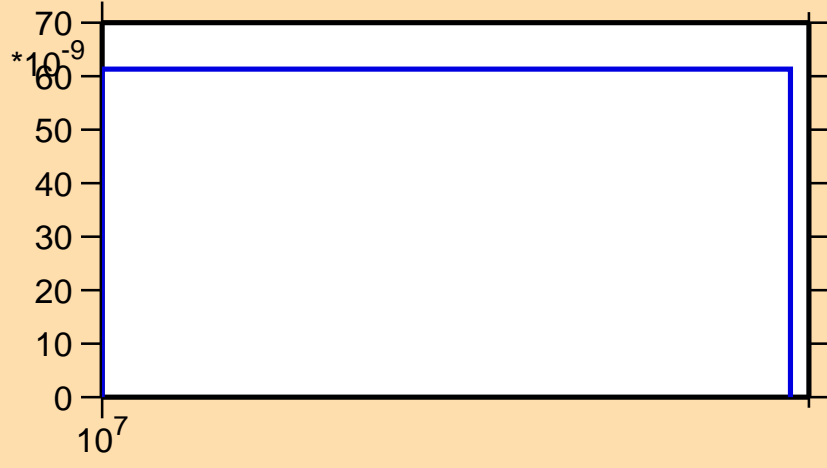
\sigma vs. E for ^{253}\text{Fm}(n,nd)
