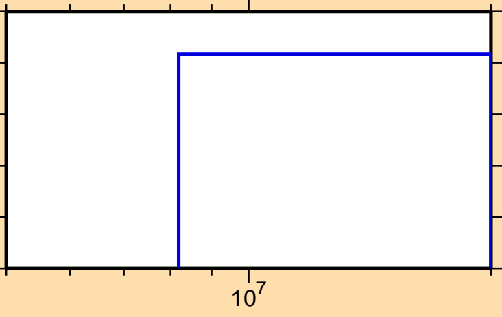
\sigma vs. E for ^{253}\text{Fm}(\text{mt117})
