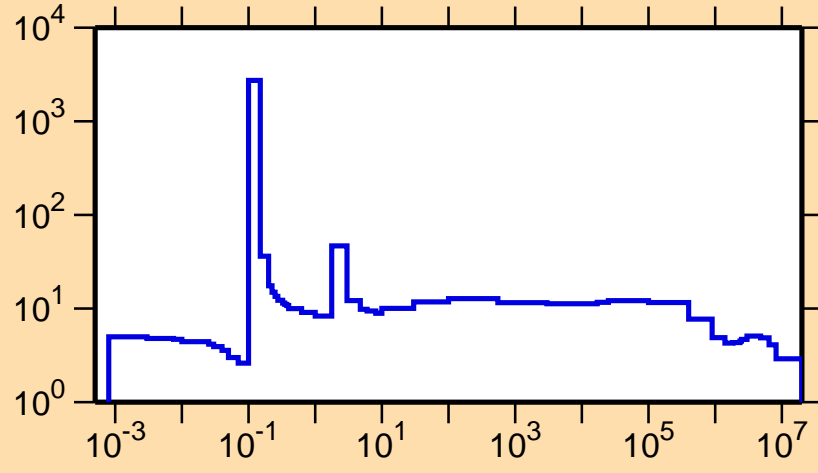
\sigma vs. E for ^{253}\text{Fm}(n,\text{el.})
