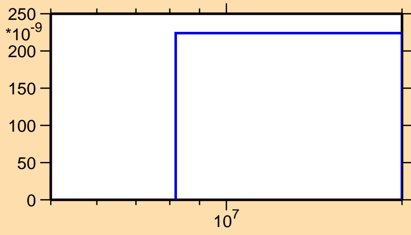
\sigma vs. E for ^{253}\text{Fm} (mt 45)
