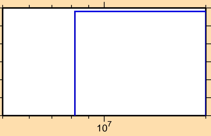
\sigma vs. E for ^{253}\text{Fm}(n,nt)
