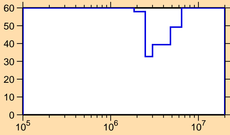
\Delta\sigma/\sigma vs. E for ^{253}\text{Fm}(n,ncont.)
