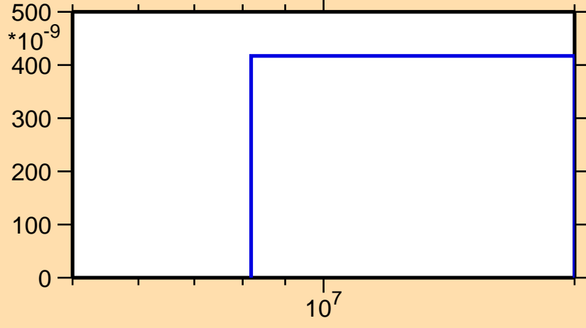
\sigma vs. E for ^{253}\text{Fm}(\text{mt117})
