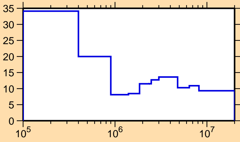
\Delta\sigma/\sigma vs. E for ^{253}\text{Fm}(n, tot.)
