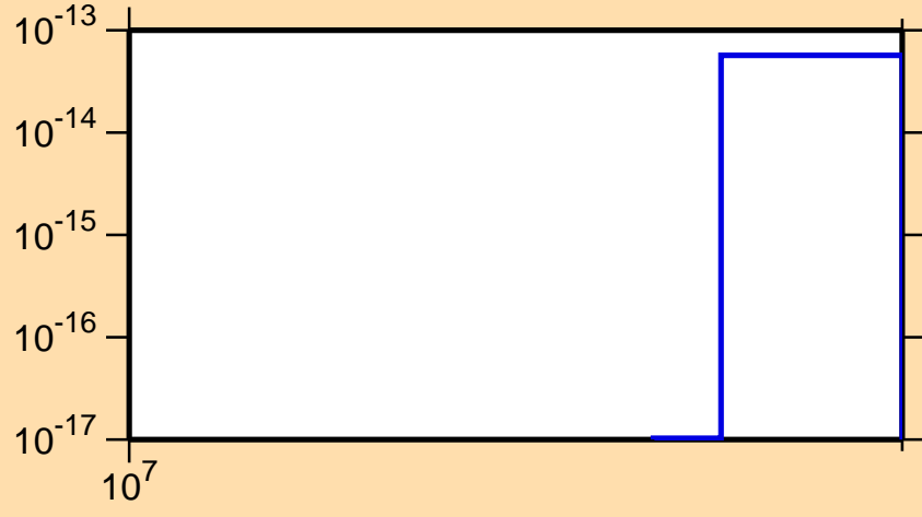
\sigma vs. E for ^{254}\text{Fm} (mt 11)
