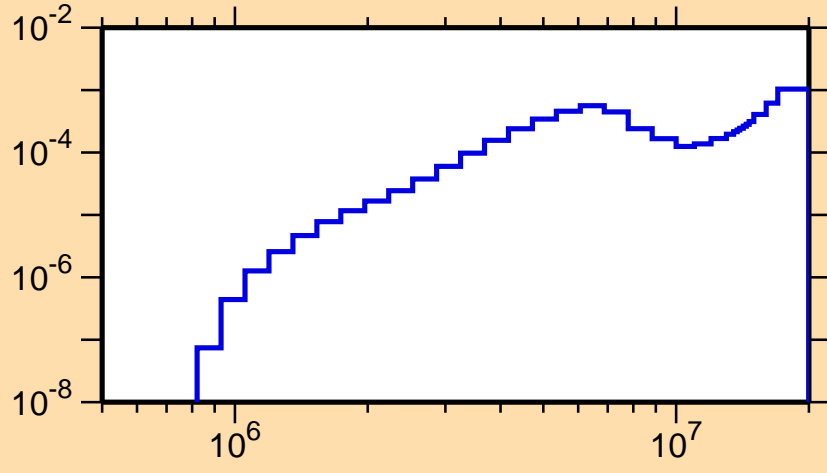
\sigma vs. E for ^{254}\text{Fm}(n,n\alpha)
