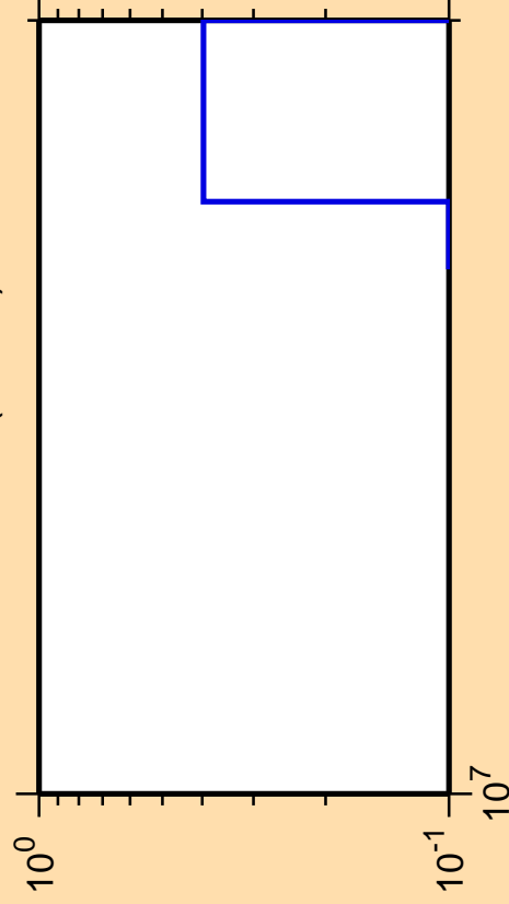
\Delta\sigma/\sigma vs. E for ^{254}\text{Fm} (mt 11)
