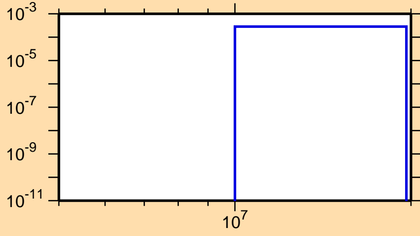
\sigma vs. E for ^{254}\text{Fm}(n,3n\alpha)
