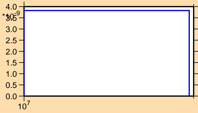
\sigma vs. E for ^{254}\text{Fm}(n,\text{nd})
