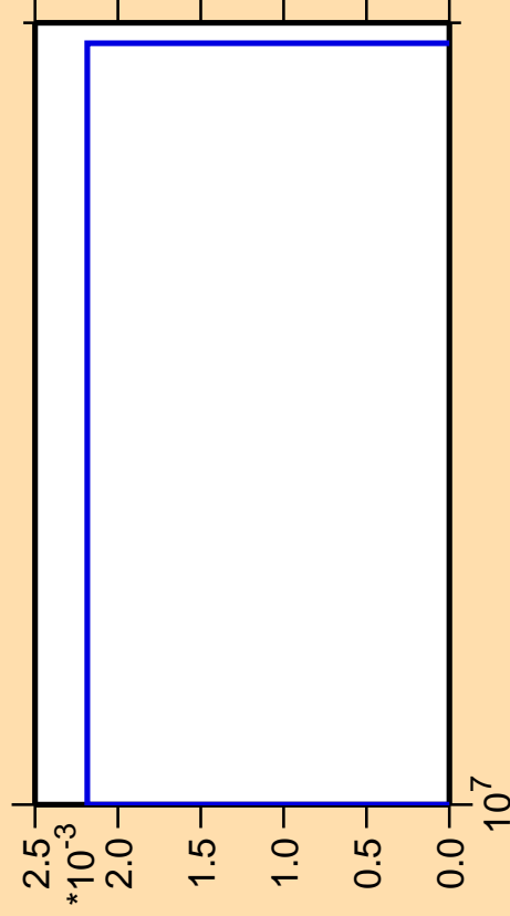
\Delta\sigma/\sigma vs. E for ^{254}\text{Fm} (mt 11)
