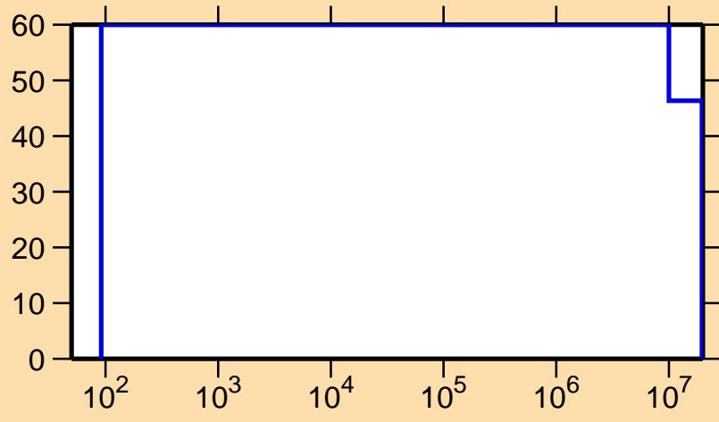
\Delta\sigma/\sigma vs. E for ^{254}\text{Fm}(n,\gamma)
