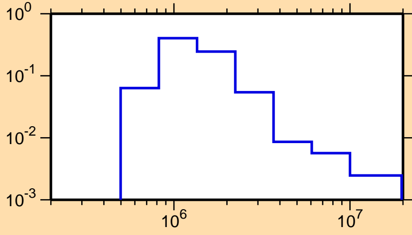
\sigma vs. E for ^{254}\text{Fm}(n,n_3)
