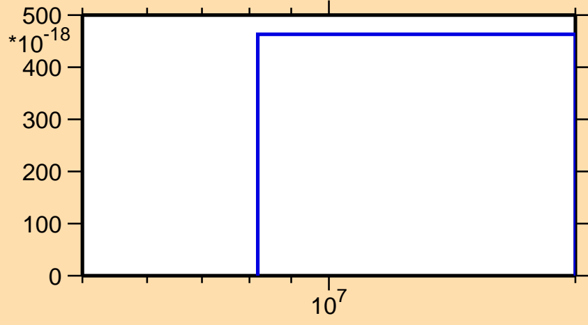
\sigma vs. E for ^{254}\text{Fm}(\text{mt } 11)
