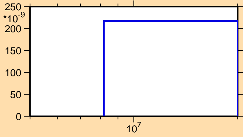
\sigma vs. E for ^{254}\text{Fm}(\text{mt117})
