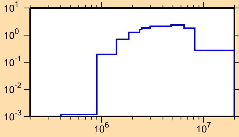
\sigma vs. E for ^{254}\text{Fm}(n,n\text{cont.})
