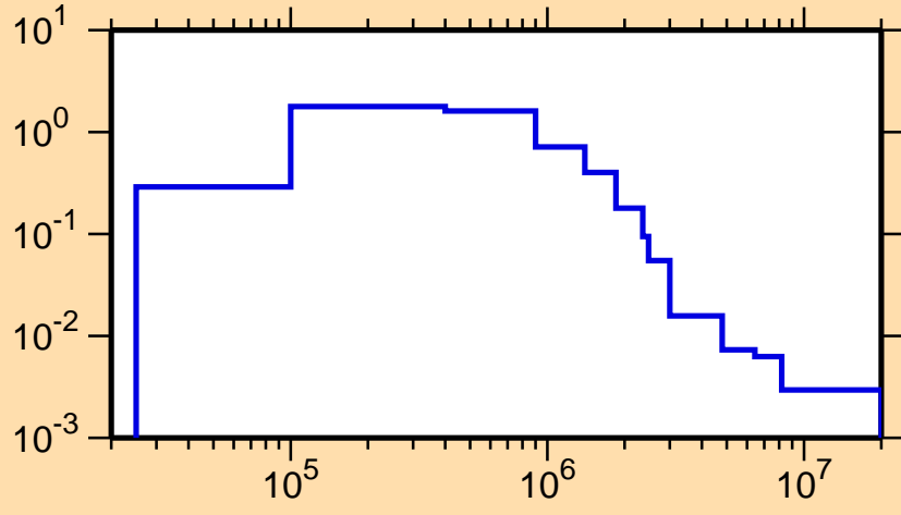
\sigma vs. E for ^{254}\text{Fm}(n,n_1)
