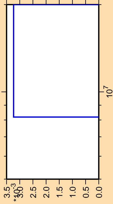
\Delta\sigma/\sigma vs. E for ^{254}\text{Fm}(\text{mt } 11)
