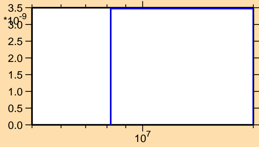
\sigma vs. E for ^{254}\text{Fm}(n,nd)
