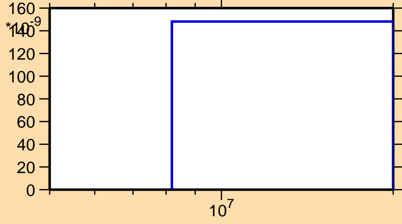
\sigma vs. E for ^{254}\text{Fm} (mt 45)
