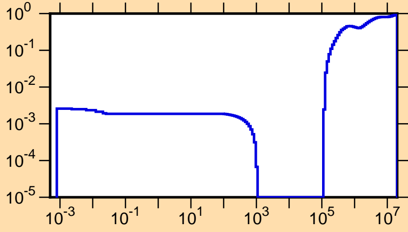
\mu vs. E for ^{255}\text{Fm}(\text{mt251})
