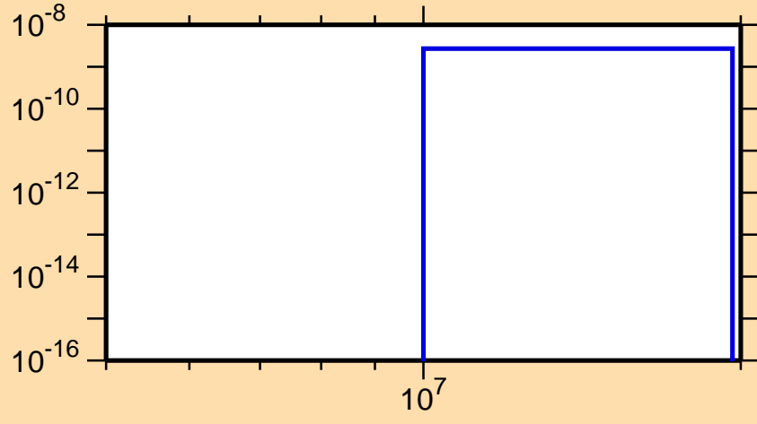
\sigma vs. E for ^{255}\text{Fm} (mt 45)
