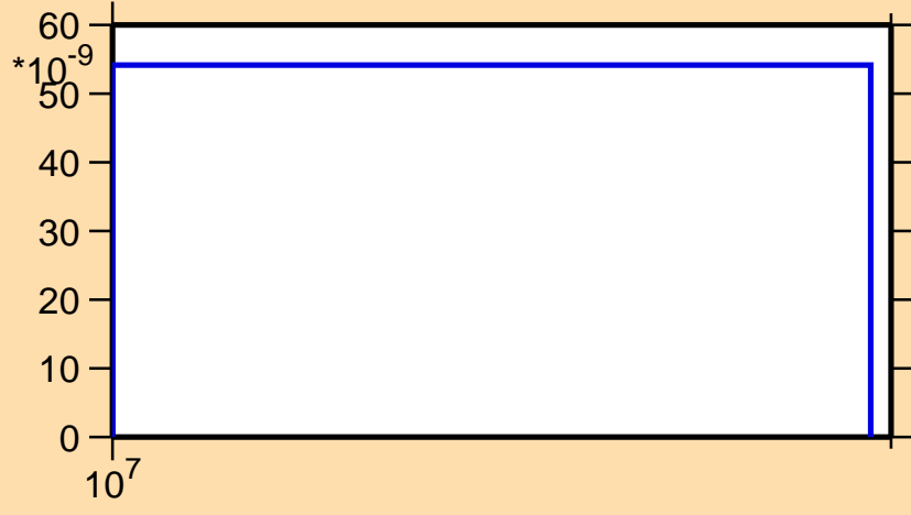
\sigma vs. E for ^{255}\text{Fm}(n,\text{nd})
