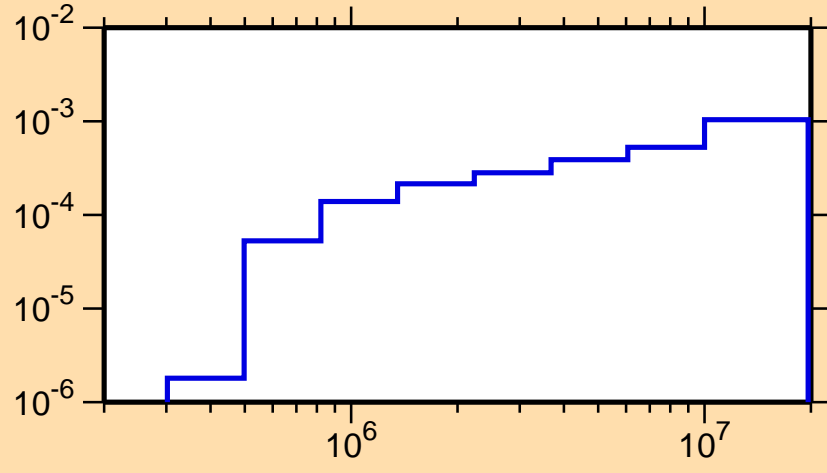
\sigma vs. E for ^{255}\text{Fm}(n,n\alpha)
