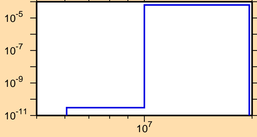
\sigma vs. E for ^{255}\text{Fm}(n,t)
