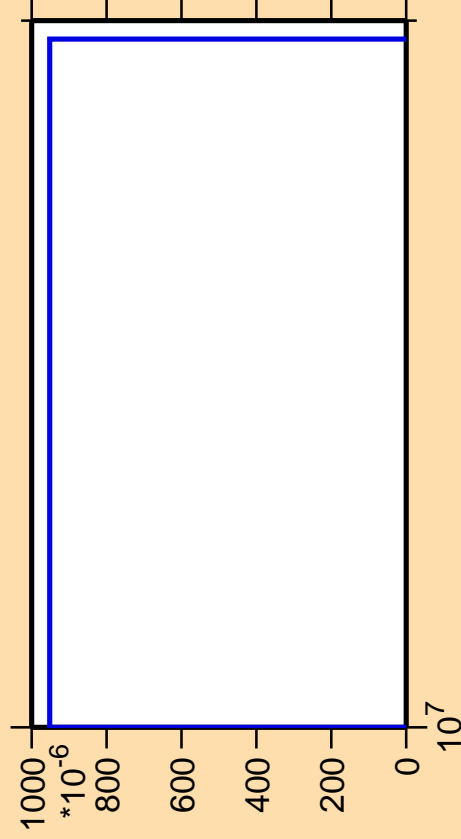
\Delta\sigma/\sigma vs. E for ^{255}\text{Fm} (mt 11)
