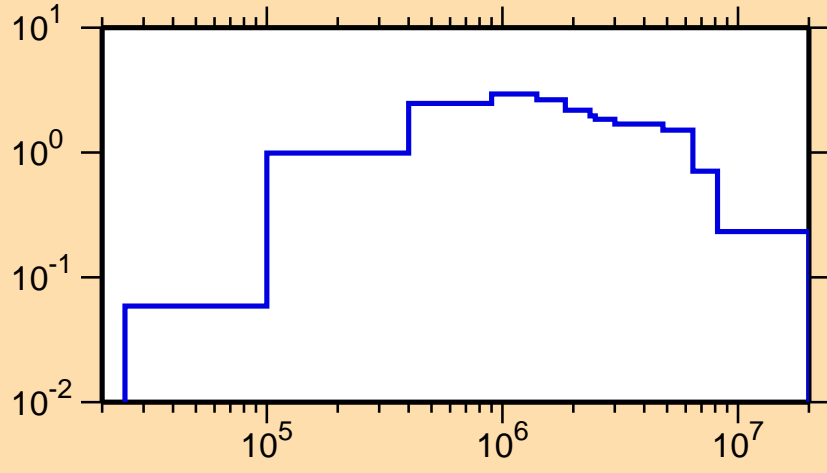
\sigma vs. E for ^{255}\text{Fm}(n,\text{inel.})
