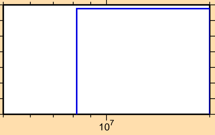
\sigma vs. E for ^{255}\text{Fm}(\text{mt117})
