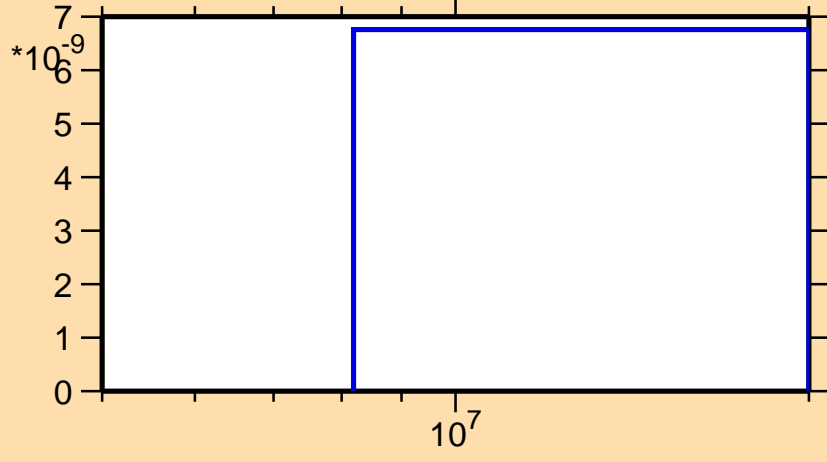
\sigma vs. E for ^{255}\text{Fm}(\text{mt117})
