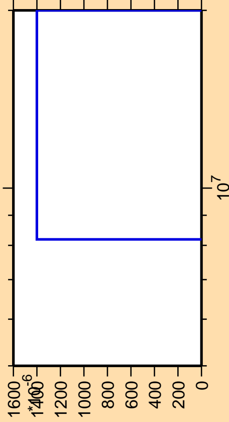
\Delta\sigma/\sigma vs. E for ^{255}\text{Fm}(\text{mt } 11)
