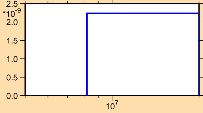
\sigma vs. E for ^{255}\text{Fm} (mt 45)
