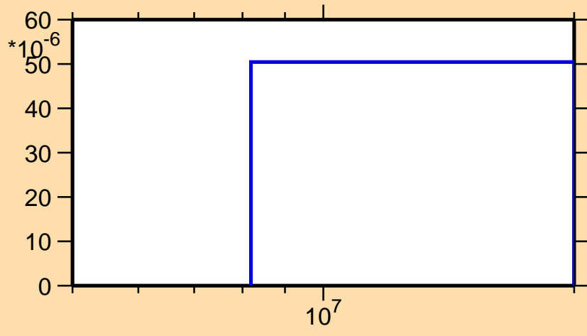
\sigma vs. E for ^{255}\text{Fm}(n,np)
