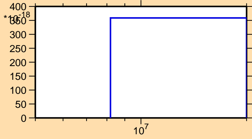
\sigma vs. E for ^{255}\text{Fm}(\text{mt } 11)
