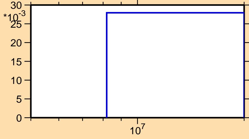
\sigma vs. E for ^{255}\text{Fm}(n,3n\alpha)
