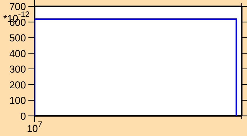
\sigma vs. E for ^{256}\text{Fm}(n,2np)
