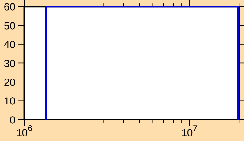
\Delta\sigma/\sigma vs. E for ^{256}\text{Fm}(n,n_1)
