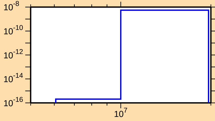
\sigma vs. E for ^{256}\text{Fm}(\text{mt } 45)
