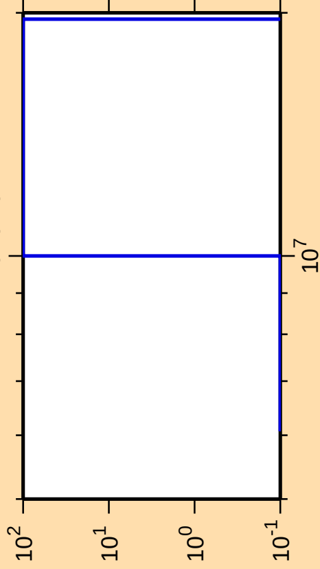
\Delta\sigma/\sigma vs. E for ^{256}\text{Fm}(n,p\alpha)
