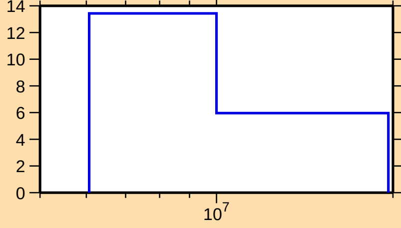
\Delta\sigma/\sigma vs. E for ^{256}\text{Fm}(n,\text{tot.})
