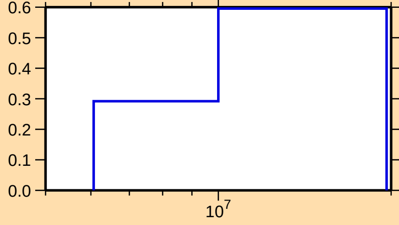
\sigma vs. E for ^{256}\text{Fm}(n,2n)
