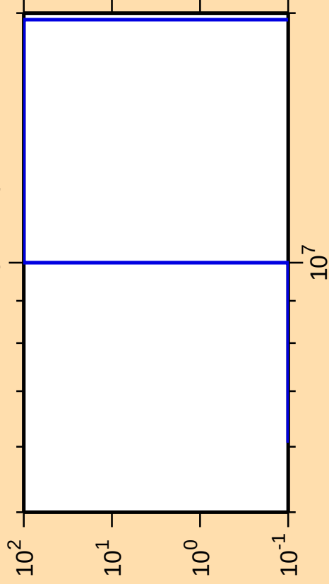
\Delta\sigma/\sigma vs. E for ^{256}\text{Fm}(\text{mt } 45)
