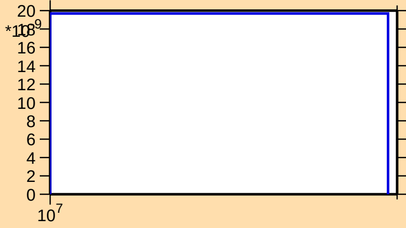
\sigma vs. E for ^{256}\text{Fm}(n,nt)
