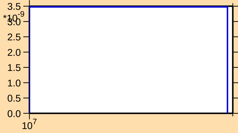
\sigma vs. E for ^{256}\text{Fm}(n,nd)
