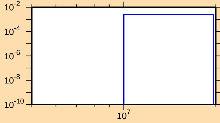
\sigma vs. E for ^{256}\text{Fm}(n,3n\alpha)
