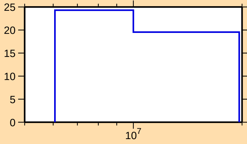
\Delta\sigma/\sigma vs. E for ^{256}\text{Fm}(n,\text{nonel.})
