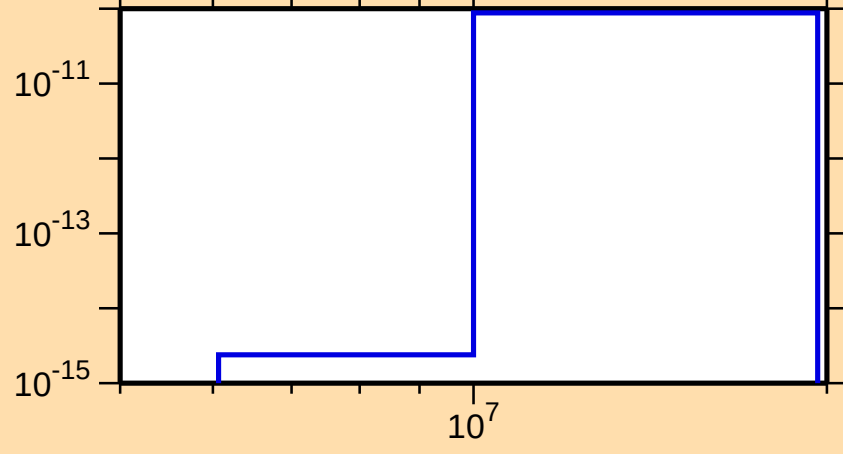
\sigma vs. E for ^{256}\text{Fm}(n,p\alpha)
