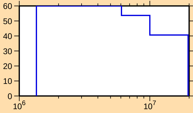
\Delta\sigma/\sigma vs. E for ^{256}\text{Fm}(n,f)
