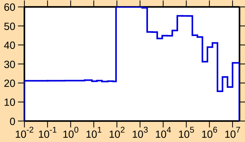
\Delta\sigma/\sigma vs. E for ^{256}\text{Fm}(n,el.)
