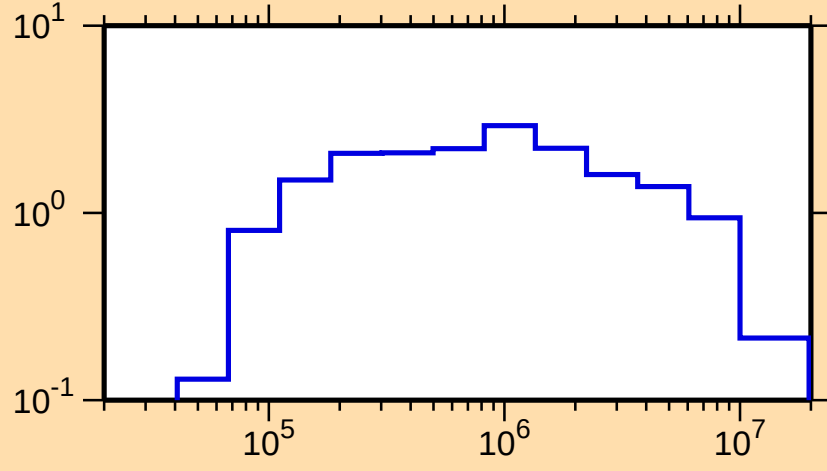
\sigma vs. E for ^{256}\text{Fm}(n,\text{inel.})
