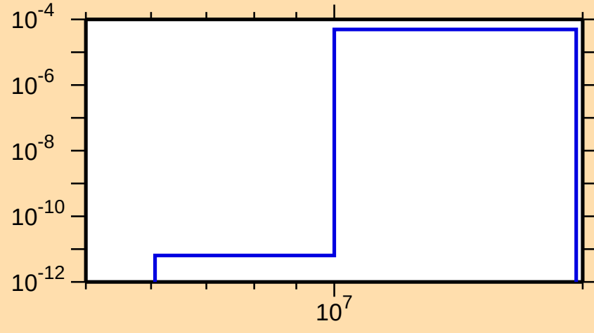
\sigma vs. E for ^{256}\text{Fm}(n,d)
