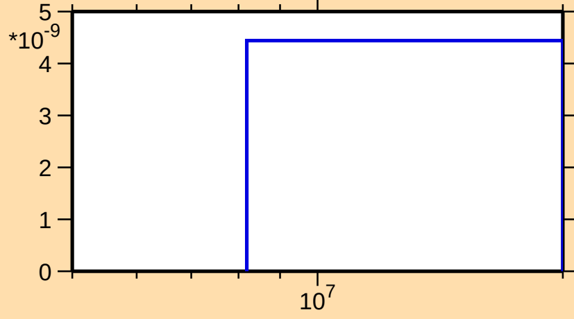
\sigma vs. E for ^{256}\text{Fm}(\text{mt } 45)
