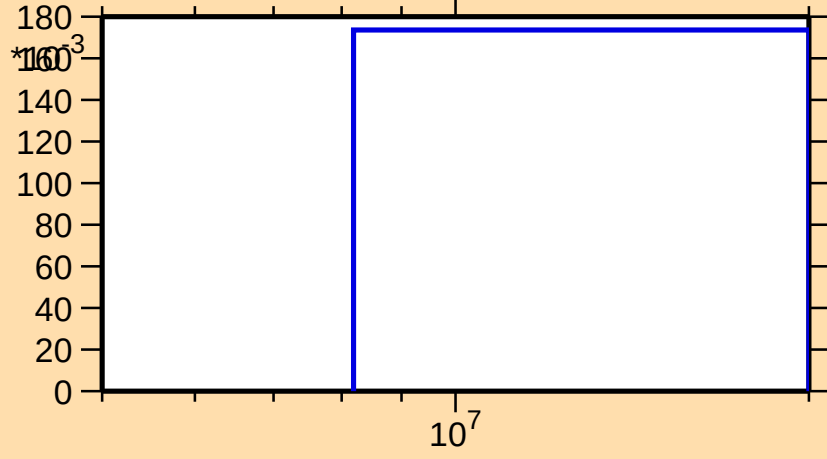
\sigma vs. E for ^{256}\text{Fm}(n,3n)
