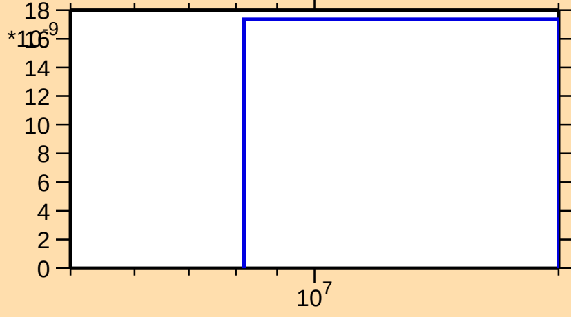
\sigma vs. E for ^{256}\text{Fm}(n,nt)
