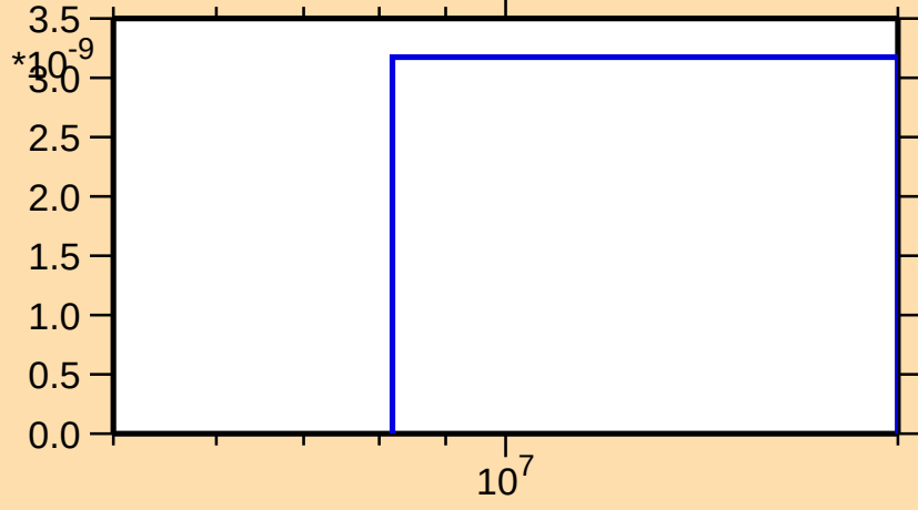
\sigma vs. E for ^{256}\text{Fm}(n,nd)
