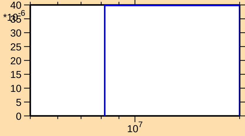
\sigma vs. E for ^{256}\text{Fm}(n,d)
