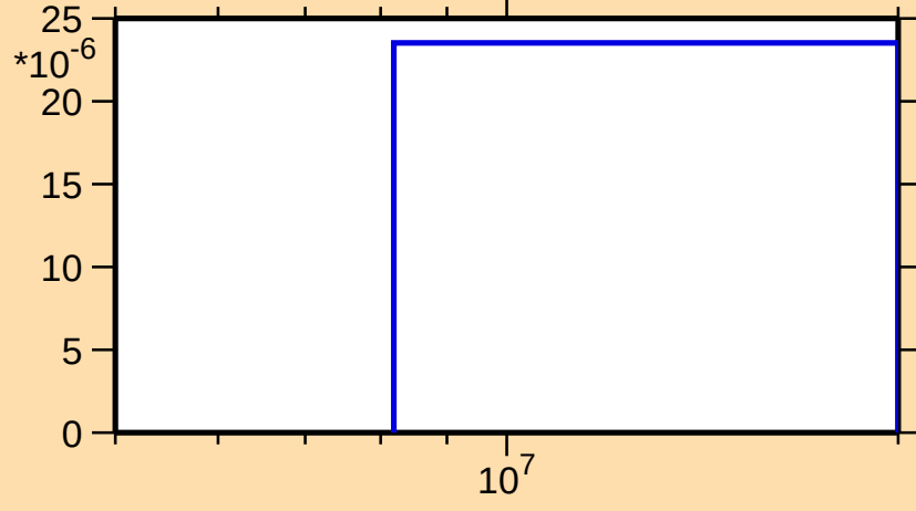
\sigma vs. E for ^{256}\text{Fm}(n,np)
