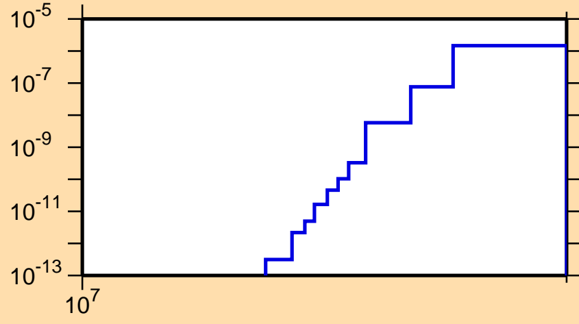
\sigma vs. E for ^{257}\text{Fm}(n,\text{nd})
