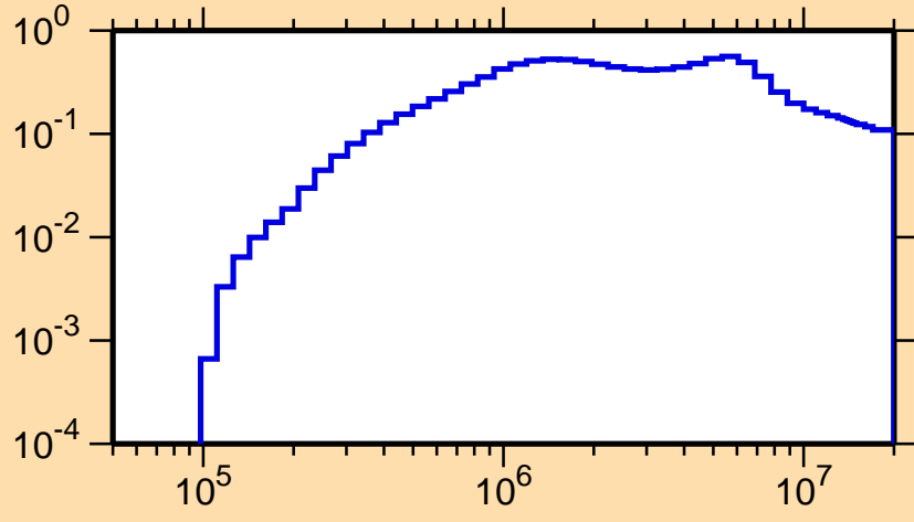
\sigma vs. E for ^{257}\text{Fm}(n,n\text{cont.})
