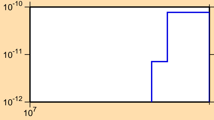
\sigma vs. E for ^{257}\text{Fm} (mt 45)
