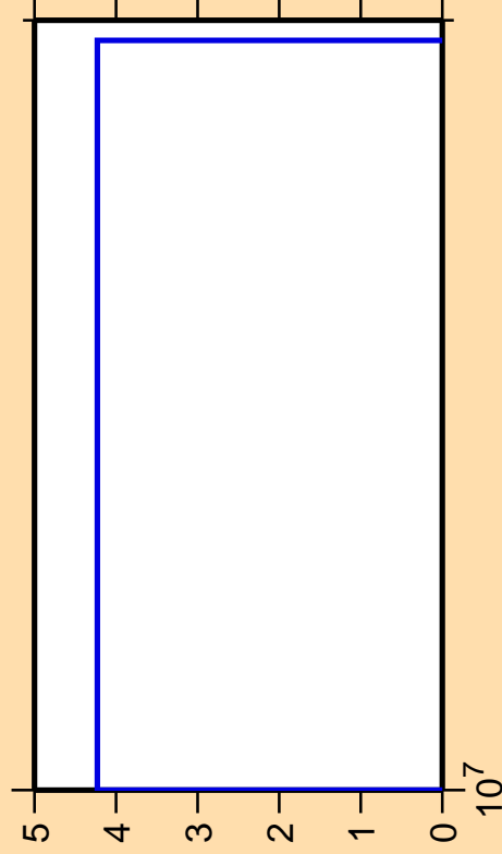
\Delta\sigma/\sigma vs. E for ^{257}\text{Fm} (mt 45)
