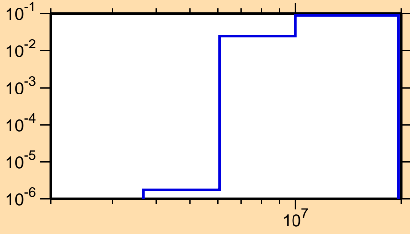
\sigma vs. E for ^{257}\text{Fm}(n,2n\alpha)
