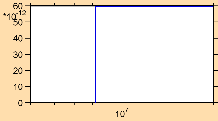
\sigma vs. E for ^{257}\text{Fm}(n,p\alpha)
