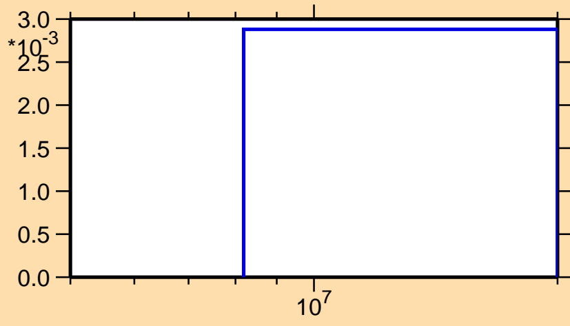
\sigma vs. E for ^{257}\text{Fm}(n,3n\alpha)
