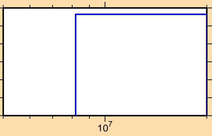
\sigma vs. E for ^{257}\text{Fm}(n,np)
