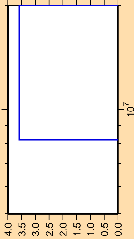
\Delta\sigma/\sigma vs. E for ^{257}\text{Fm} (mt 45)
