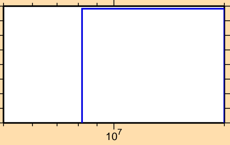
\sigma vs. E for ^{257}\text{Fm}(n,\text{nd})
