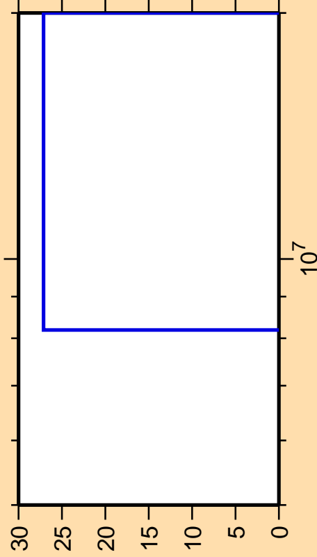
\Delta\sigma/\sigma vs. E for ^{257}\text{Fm}(\text{mt117})
