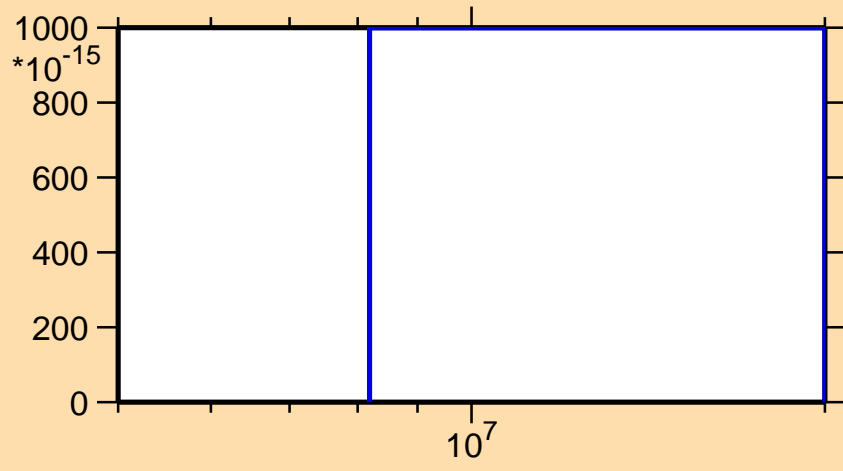
\sigma vs. E for ^{257}\text{Fm} (mt 45)
