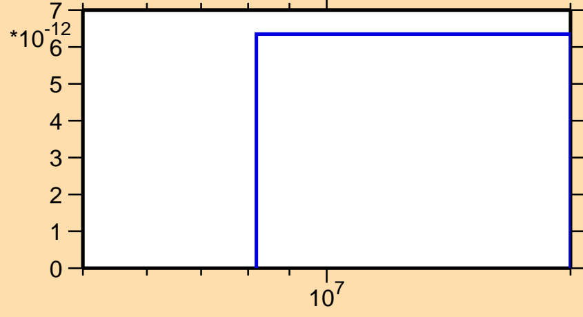
\sigma vs. E for ^{257}\text{Fm}(\text{mt117})
