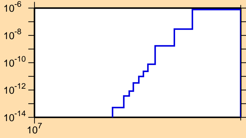
\sigma vs. E for ^{259}\text{Fm}(n,nt)
