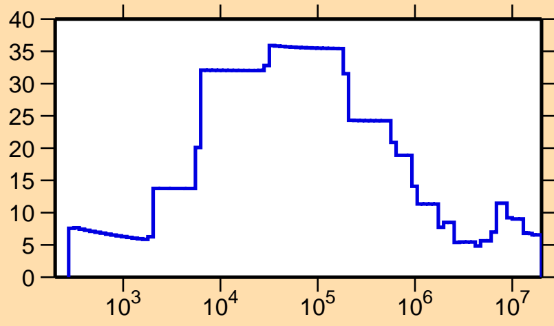
\Delta\sigma/\sigma vs. E for ^{259}\text{Fm}(n,\text{tot.})
