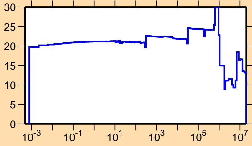
\Delta\sigma/\sigma vs. E for ^{259}\text{Fm}(n,el.)
