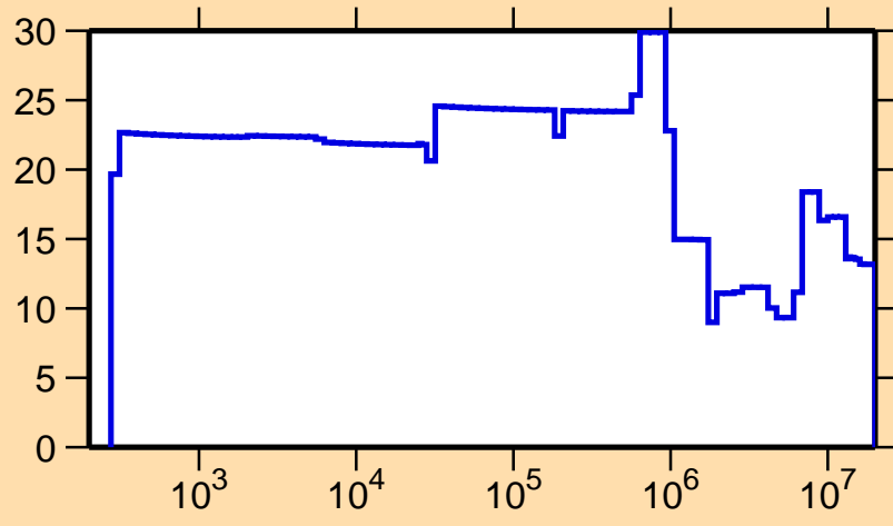
\Delta\sigma/\sigma vs. E for ^{259}\text{Fm}(n,\text{el.})
