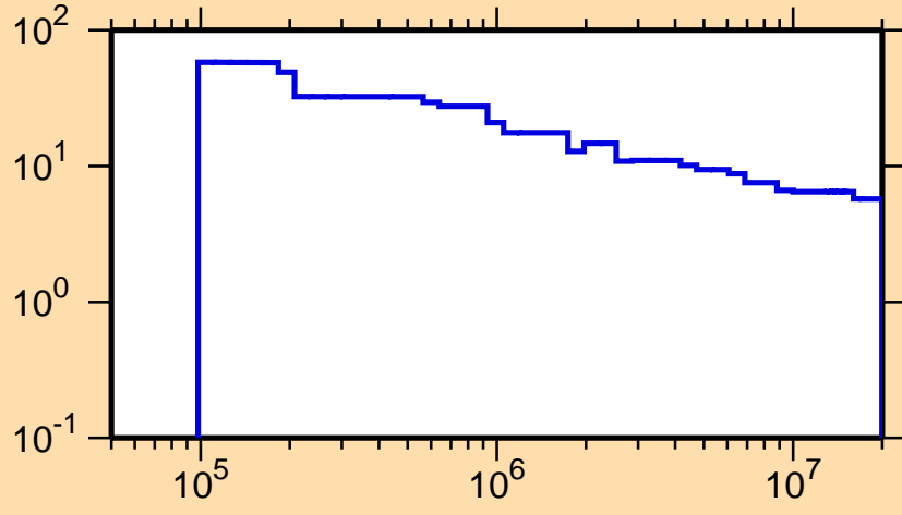
\Delta\sigma/\sigma vs. E for ^{259}\text{Fm}(n,nonel.)
