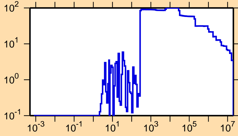
\Delta\sigma/\sigma vs. E for ^{259}\text{Fm}(n,f)
