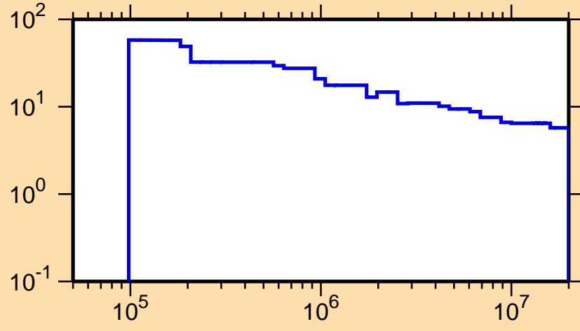
\Delta\sigma/\sigma vs. E for ^{259}\text{Fm}(n,\text{nonel.})
