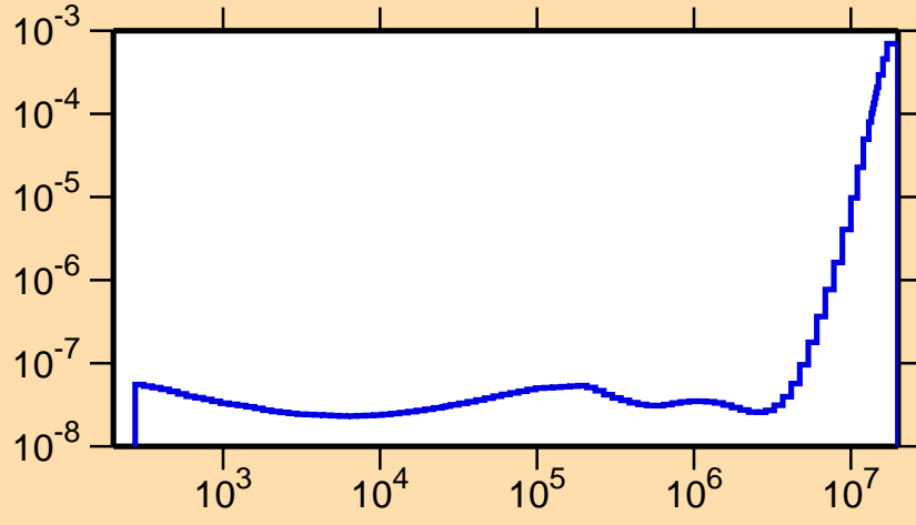
\sigma vs. E for ^{259}\text{Fm}(n,\alpha)
