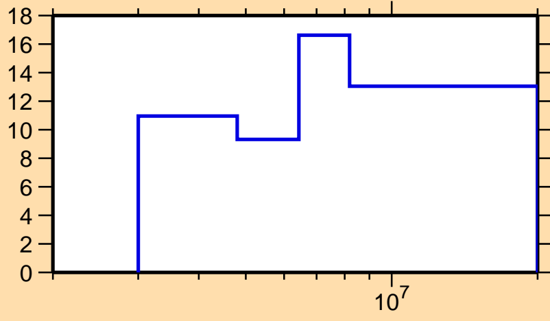
\Delta\sigma/\sigma vs. E for ^{259}\text{Fm}(n,el.)
