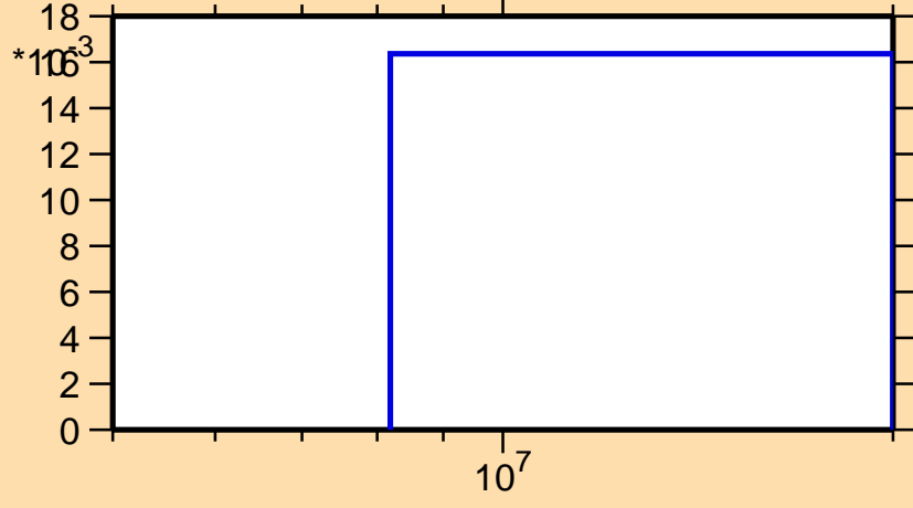
\sigma vs. E for ^{259}\text{Fm}(n,3n)
