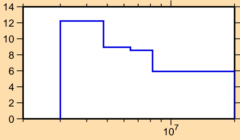
\Delta\sigma/\sigma vs. E for ^{259}\text{Fm}(n,f)
