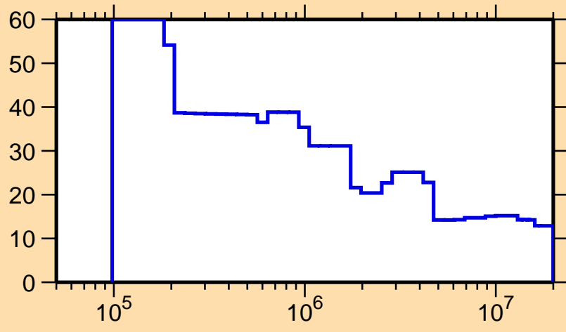
\Delta\sigma/\sigma vs. E for ^{260}\text{Fm}(n,nonel.)
