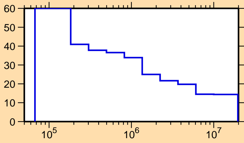
\Delta\sigma/\sigma vs. E for ^{260}\text{Fm}(n,n\text{onel.})
