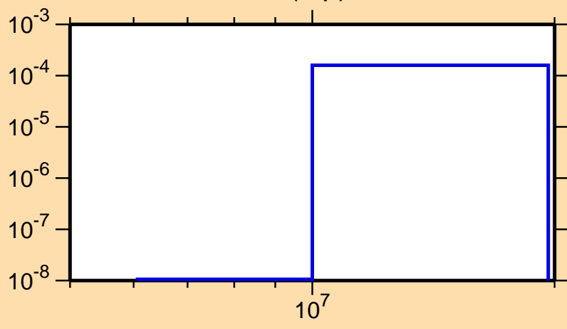
\sigma vs. E for ^{260}\text{Fm}(n,p)
