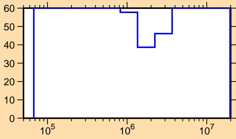
\Delta\sigma/\sigma vs. E for ^{260}\text{Fm}(n,n_1)
