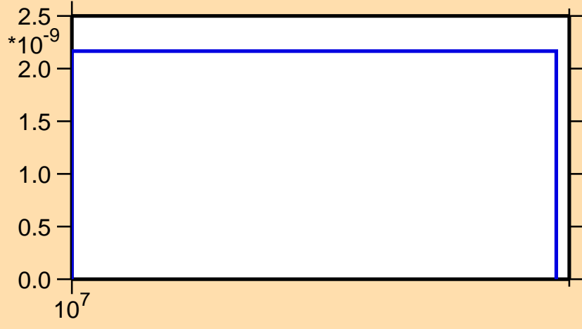
\sigma vs. E for ^{260}\text{Fm}(n,nt)
