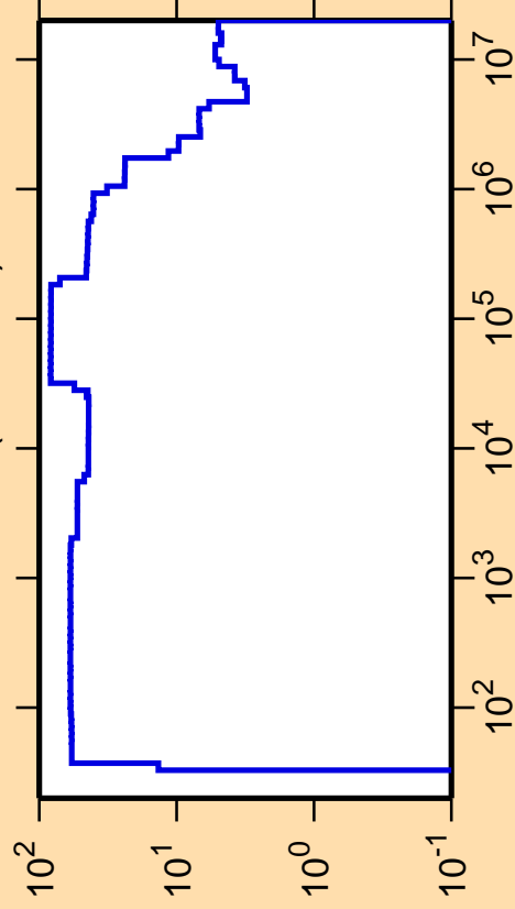
\Delta\sigma/\sigma vs. E for ^{204}\text{Fr}(n,\text{nonel.})
