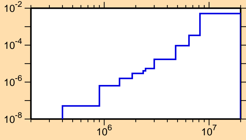
\sigma vs. E for ^{204}\text{Fr}(n,n\alpha)
