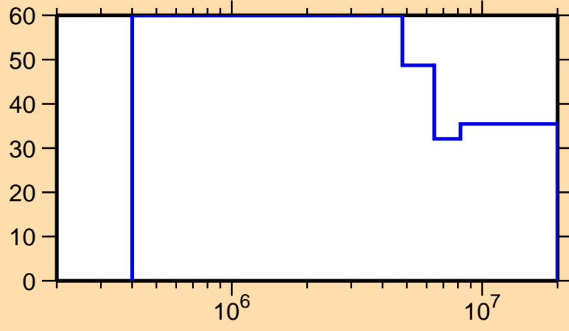
\Delta\sigma/\sigma vs. E for ^{204}\text{Fr}(n,n\text{cont.})
