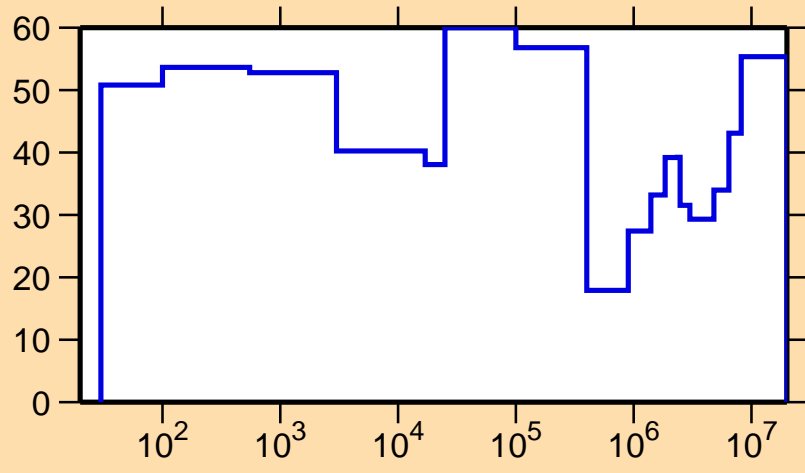
\Delta\sigma/\sigma vs. E for ^{204}\text{Fr}(n,\gamma)
