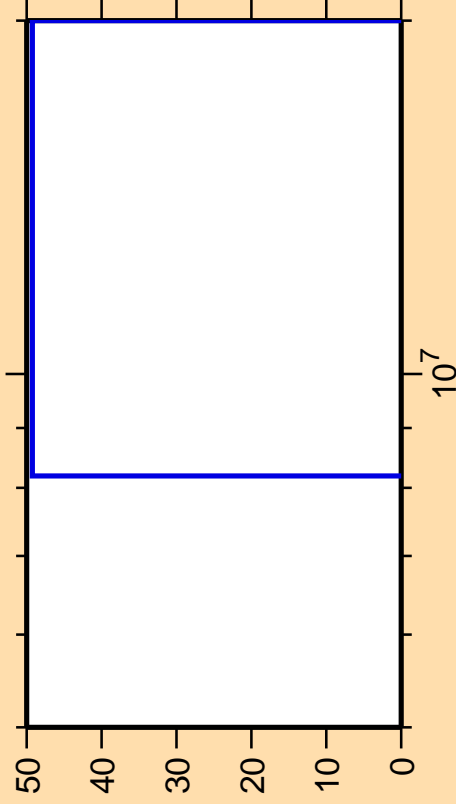
\Delta\sigma/\sigma vs. E for ^{204}\text{Fr}(n,n_1)
