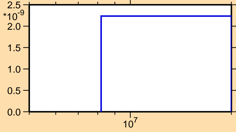
\sigma vs. E for ^{204}\text{Fr}(n,3n)
