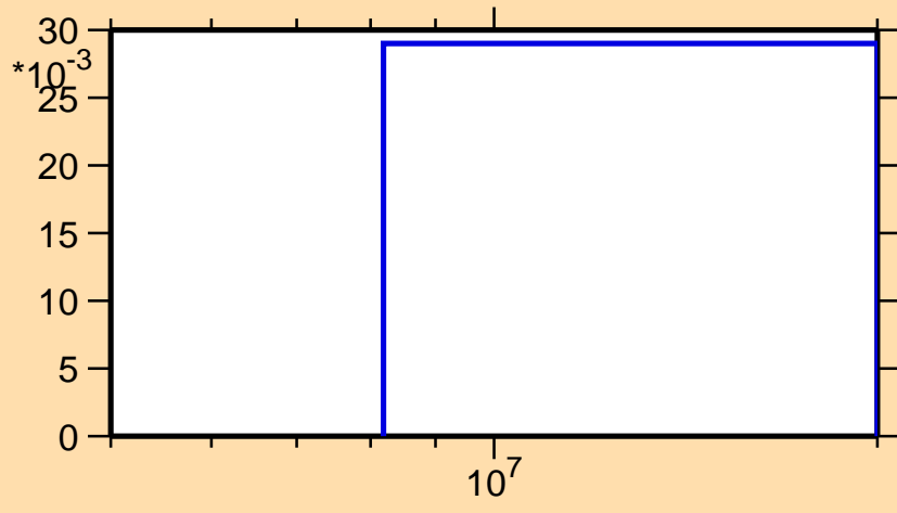
\sigma vs. E for ^{204}\text{Fr}(n,2n)
