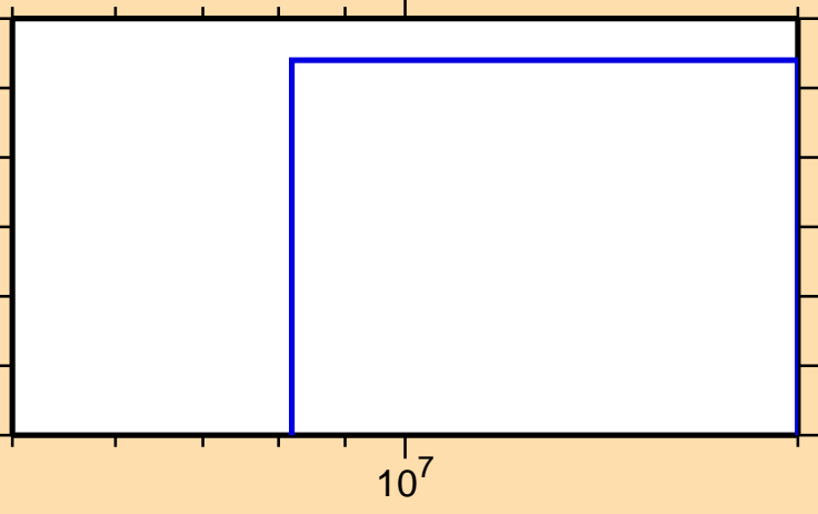
\sigma vs. E for ^{204}\text{Fr}(n,2np)
