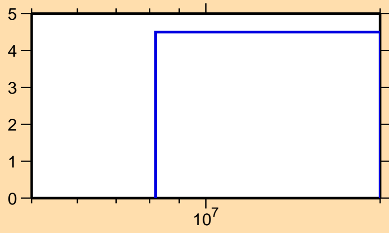
\Delta\sigma/\sigma vs. E for ^{204}\text{Fr}(n,\text{el.})
