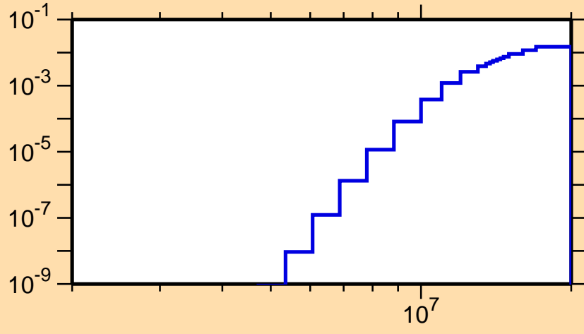
\sigma vs. E for ^{204}\text{Fr}(n,d)
