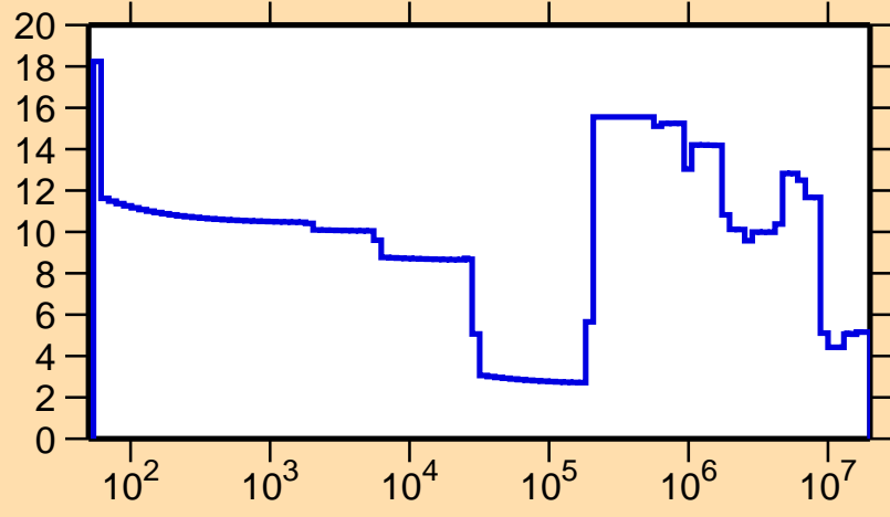
\Delta\sigma/\sigma vs. E for ^{204}\text{Fr}(n,el.)
