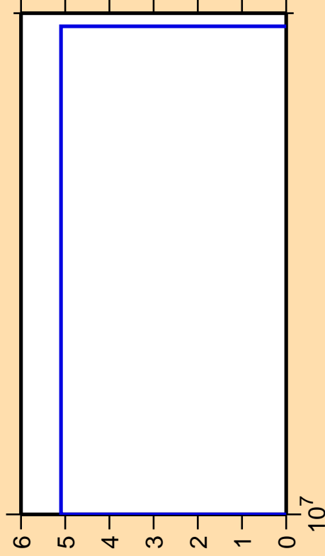
\Delta\sigma/\sigma vs. E for ^{204}\text{Fr}(\text{mt } 34)
