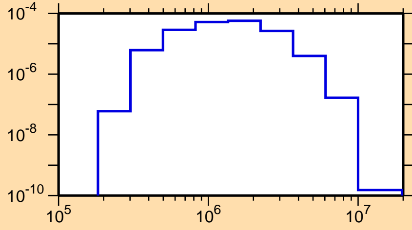
\sigma vs. E for ^{204}\text{Fr}(n,n_2)
